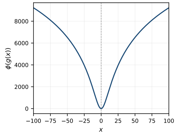
Oscillatory: \phi(u) = u(1 + 0.45\sin(0.02u))
