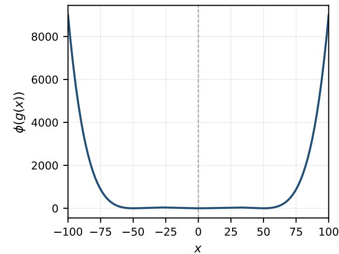
Repeated optima: \phi(u) = u(u - 2500)^2/6.25 \cdot 10^7
