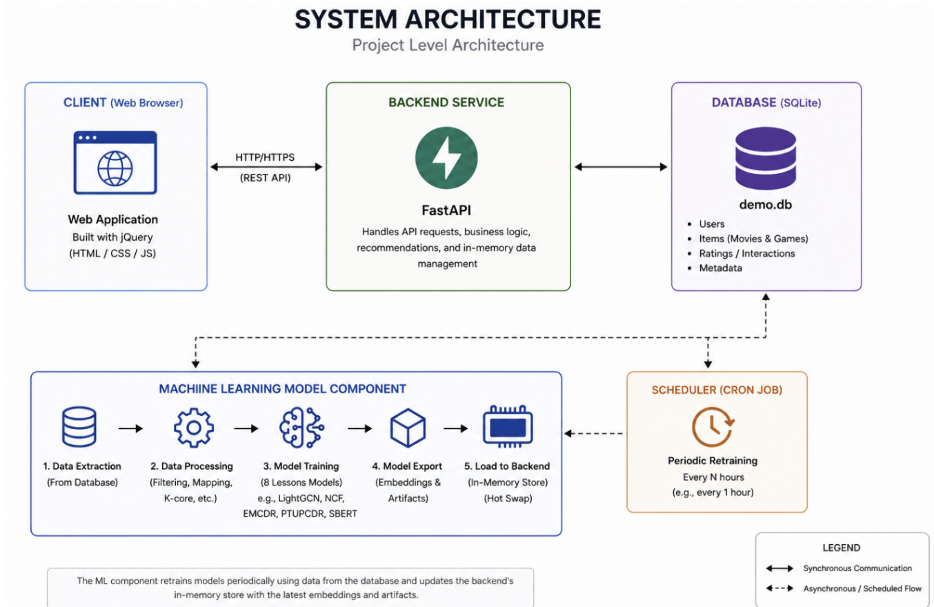
Figure 32: System architecture
