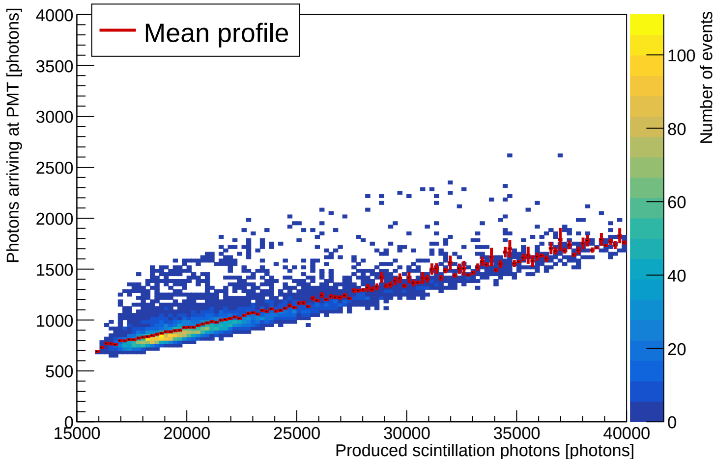
Sensor photon collection versus produced light (40x 40 mm tile)
