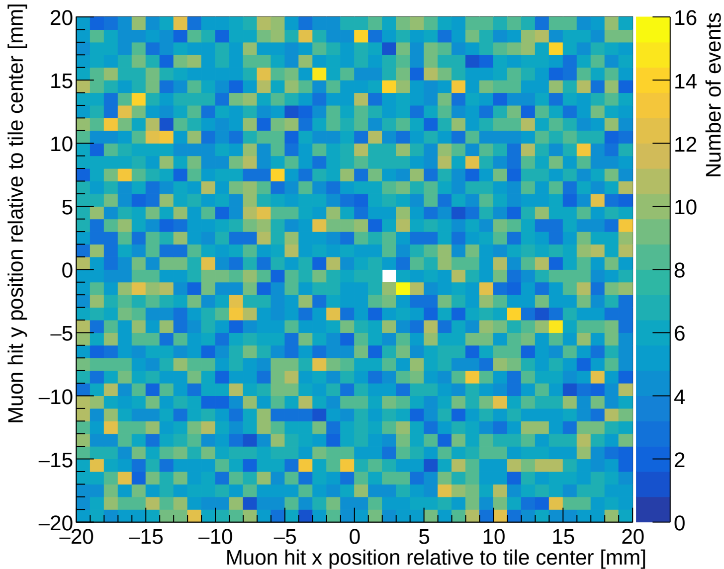
Simulated muon hit positions (40× 40 mm tile)
