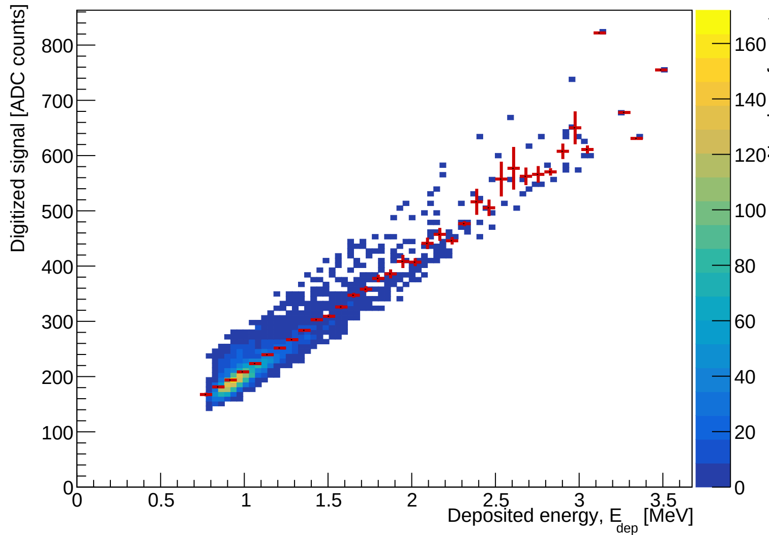
ADC response versus deposited energy (20 x 20 mm tile)
