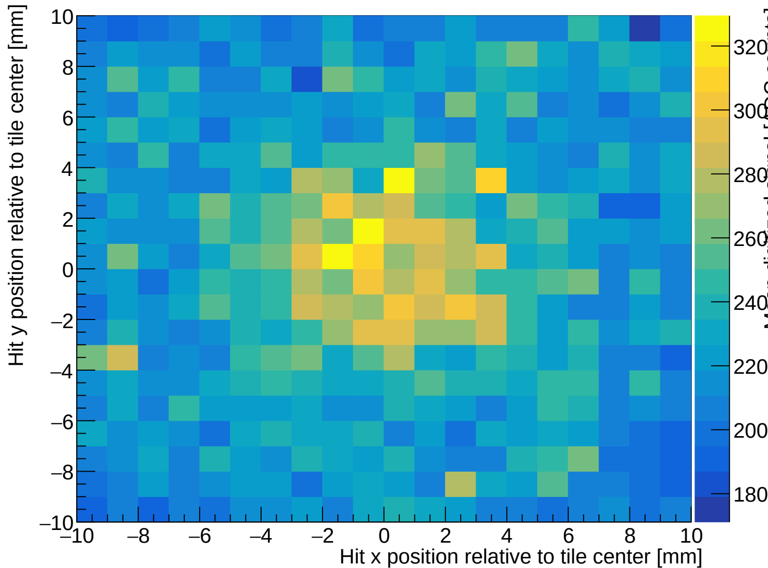
Mean ADC response versus hit position (20 x 20 mm tile)
