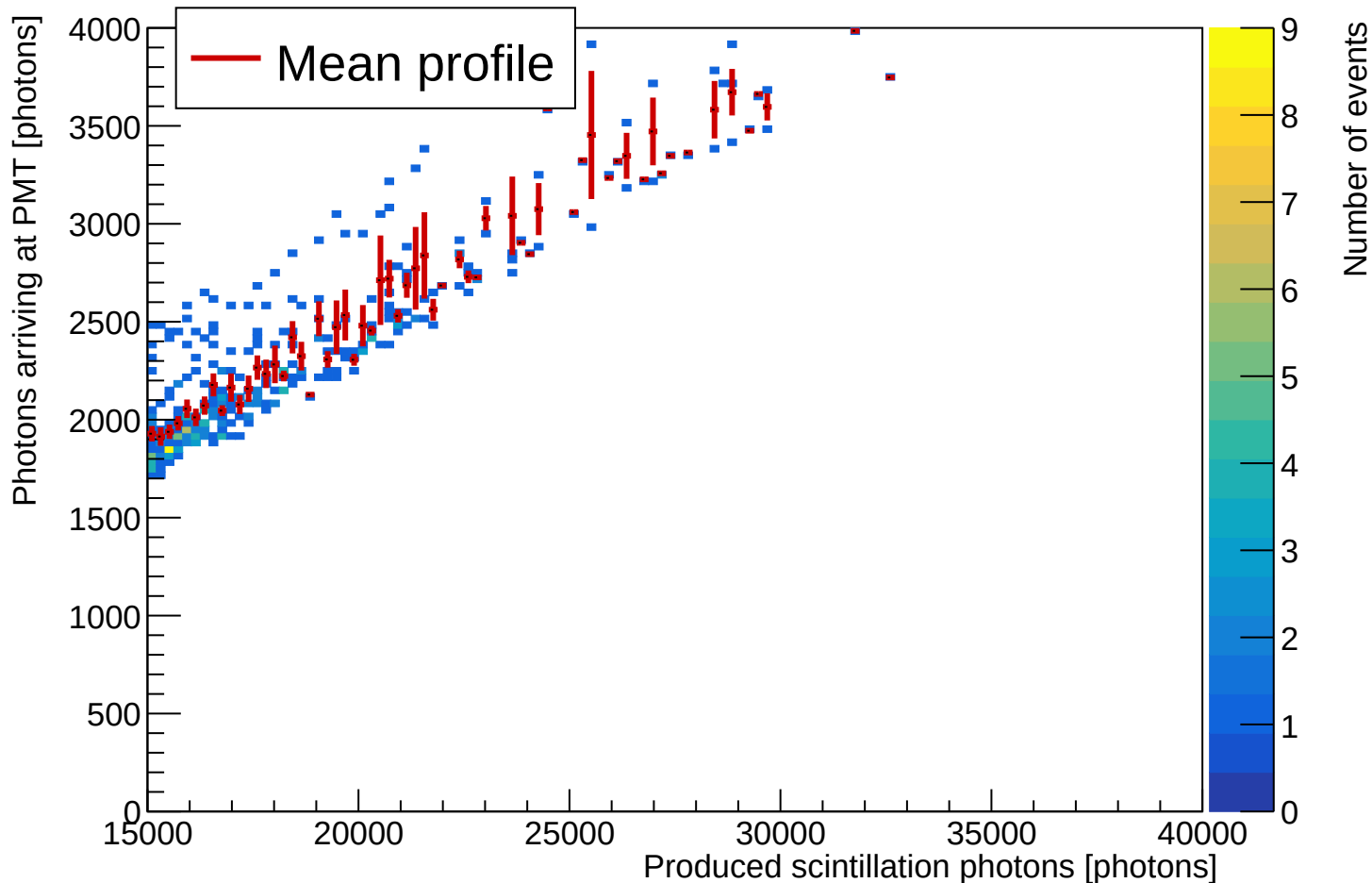
Sensor photon collection versus produced light (20x 20 mm tile)
