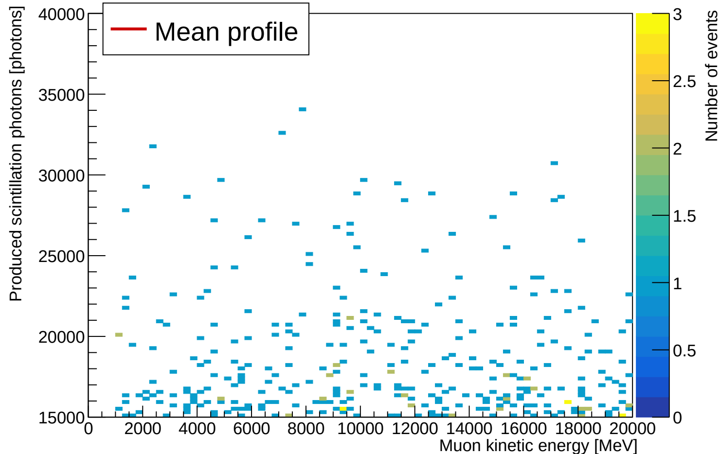
Scintillation-light production versus muon energy (20x 20 mm tile)
