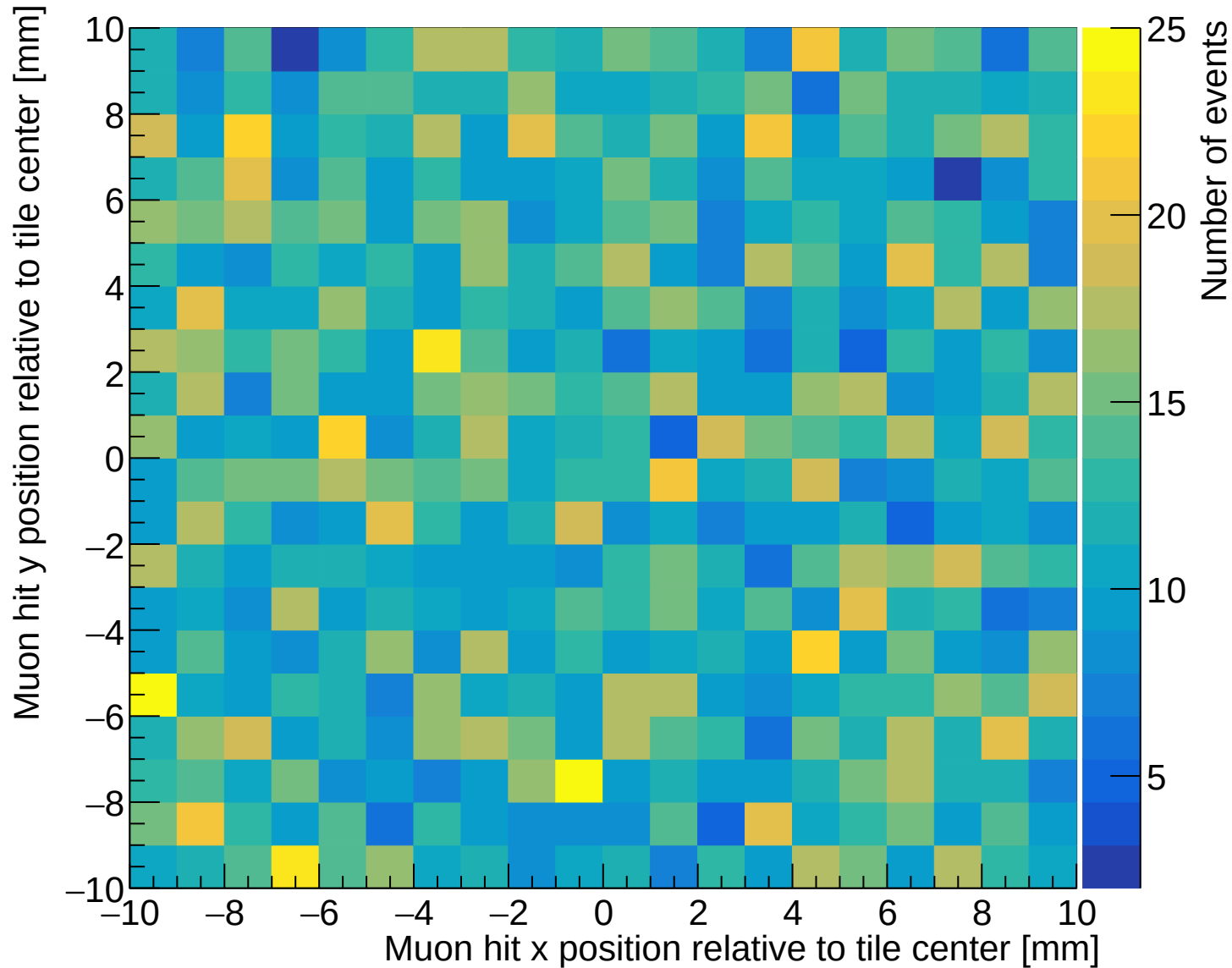
Simulated muon hit positions (20×20 mm tile)
