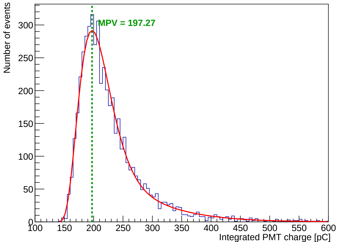
PMT charge distribution (20× 20 mm tile)
