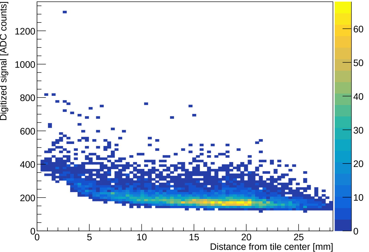
ADC response versus radial hit position (40 x 40 mm tile)
