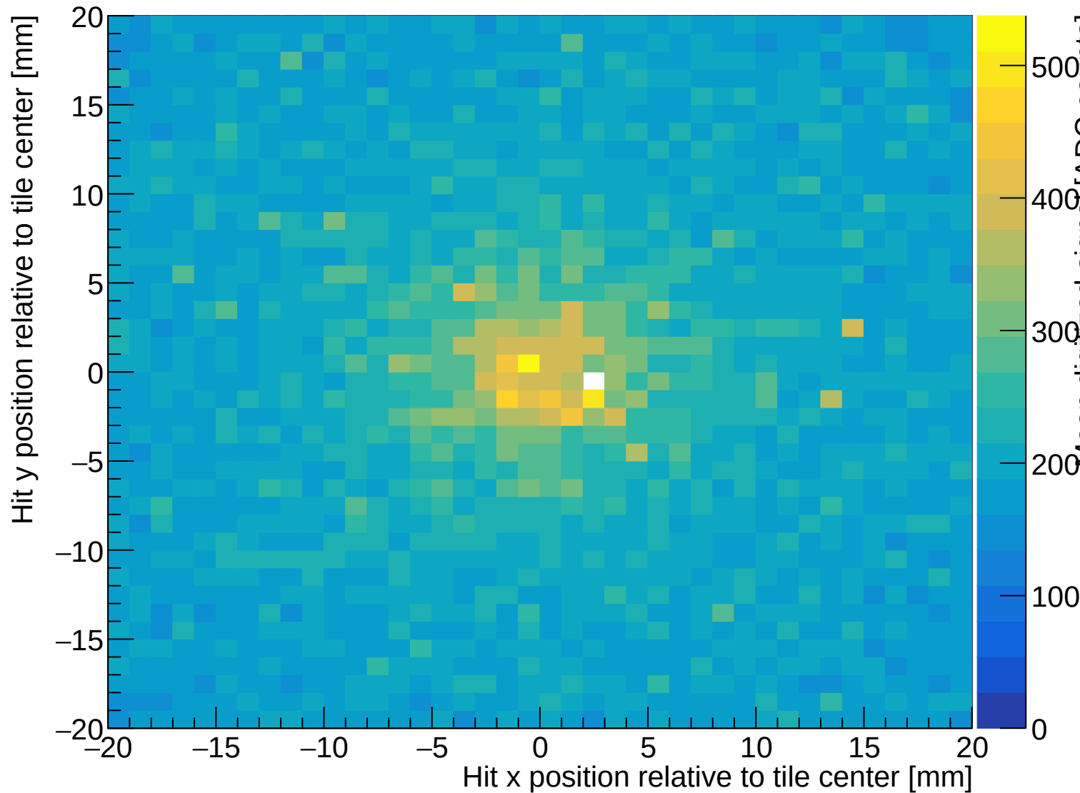
Mean ADC response versus hit position (40 x 40 mm tile)
