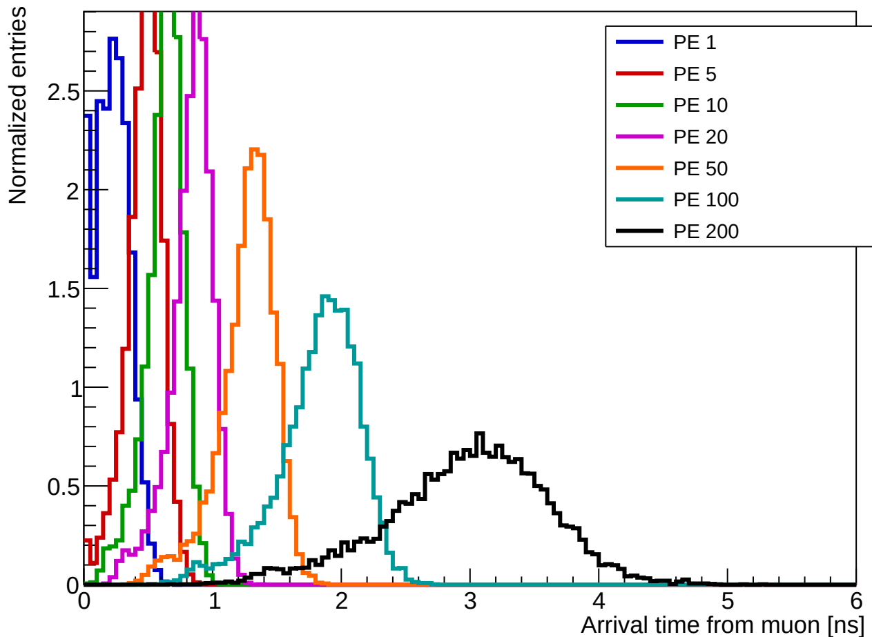
Arrival-Time Overlays for Selected Photoelectron Indices
