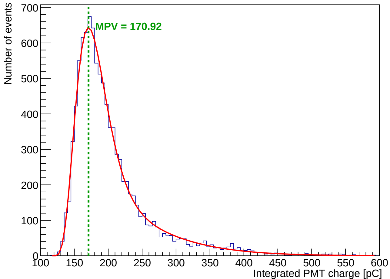
PMT charge distribution (40× 40 mm tile)
