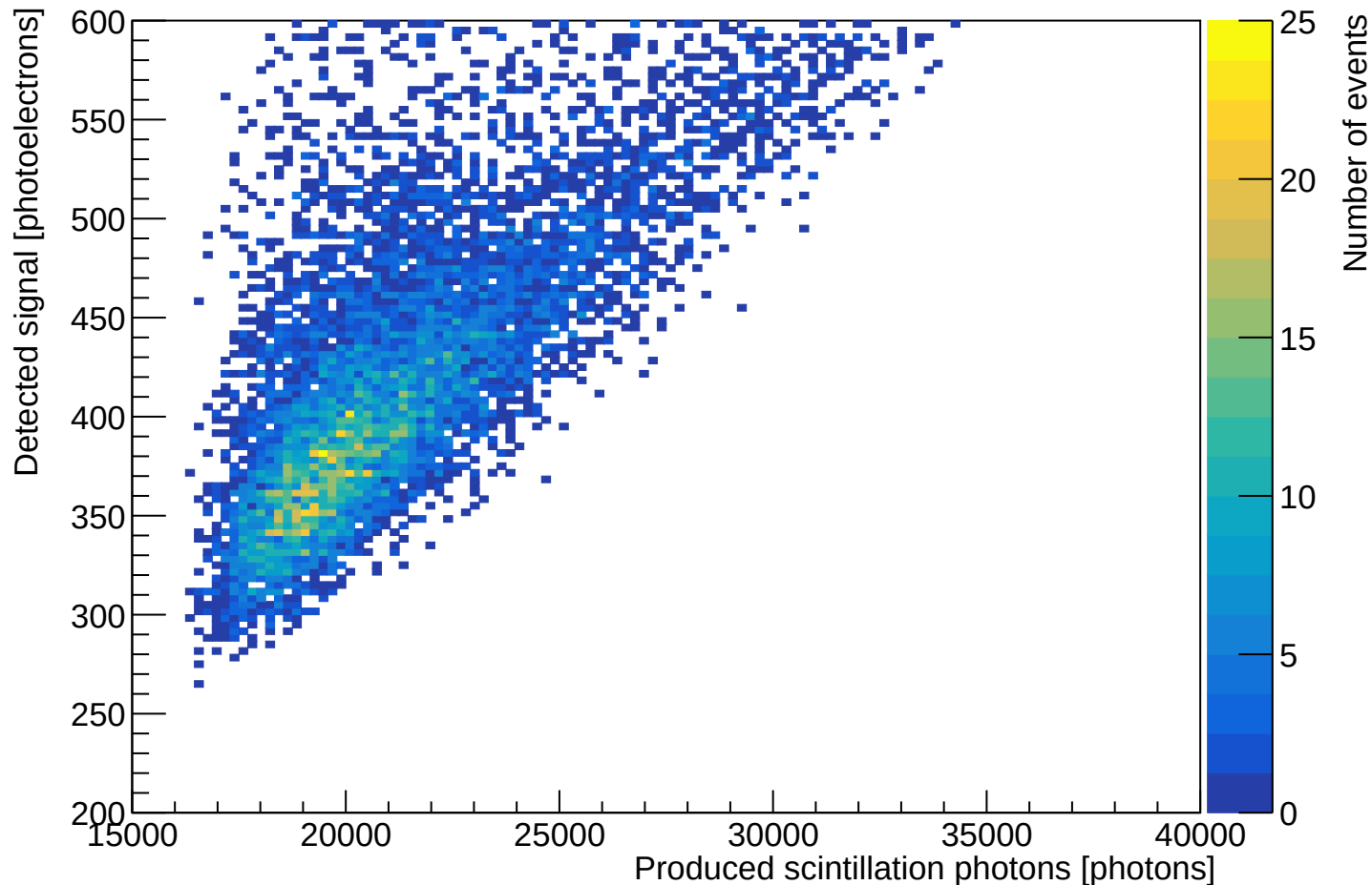
Detected photoelectrons versus produced light (40x 40 mm tile)
