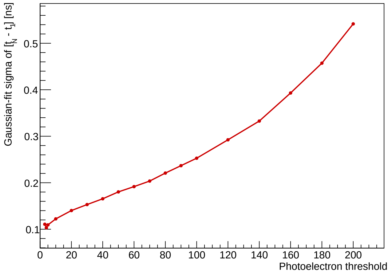
Sigma of Arrival-Time Difference vs Threshold
