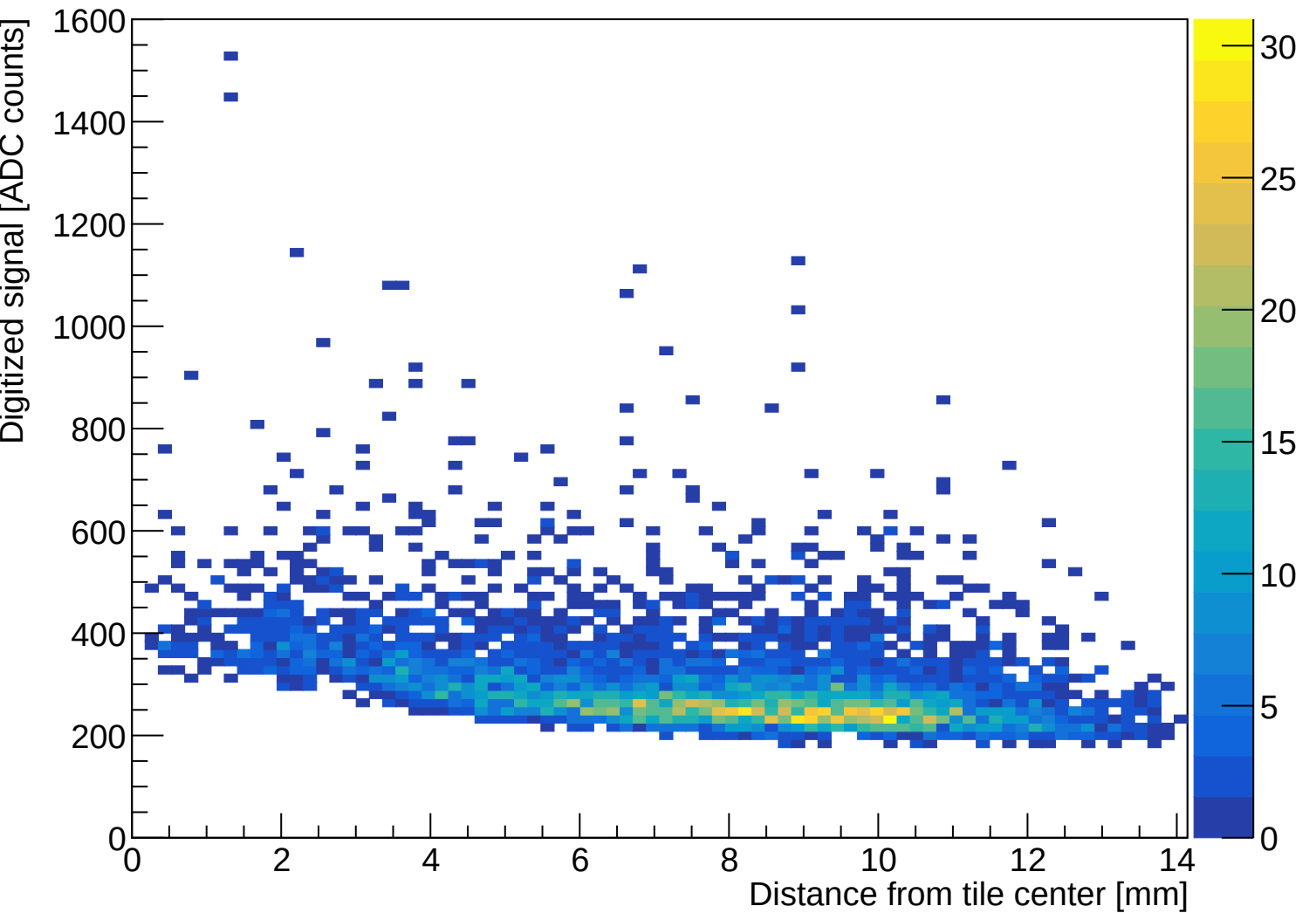
ADC response versus radial hit position (20 x 20 mm tile)
