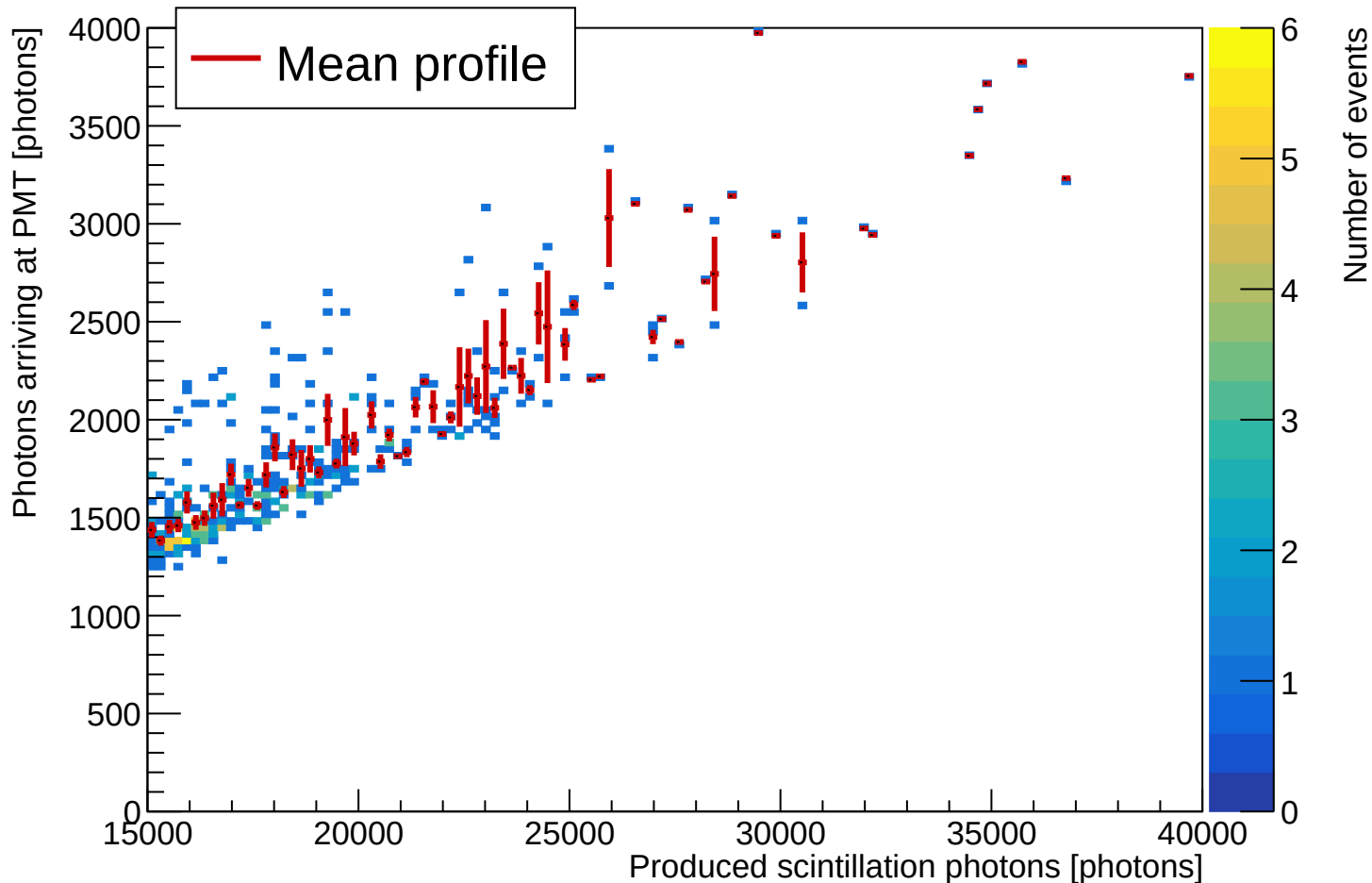
Sensor photon collection versus produced light ( 20 \times 20 mm tile)
