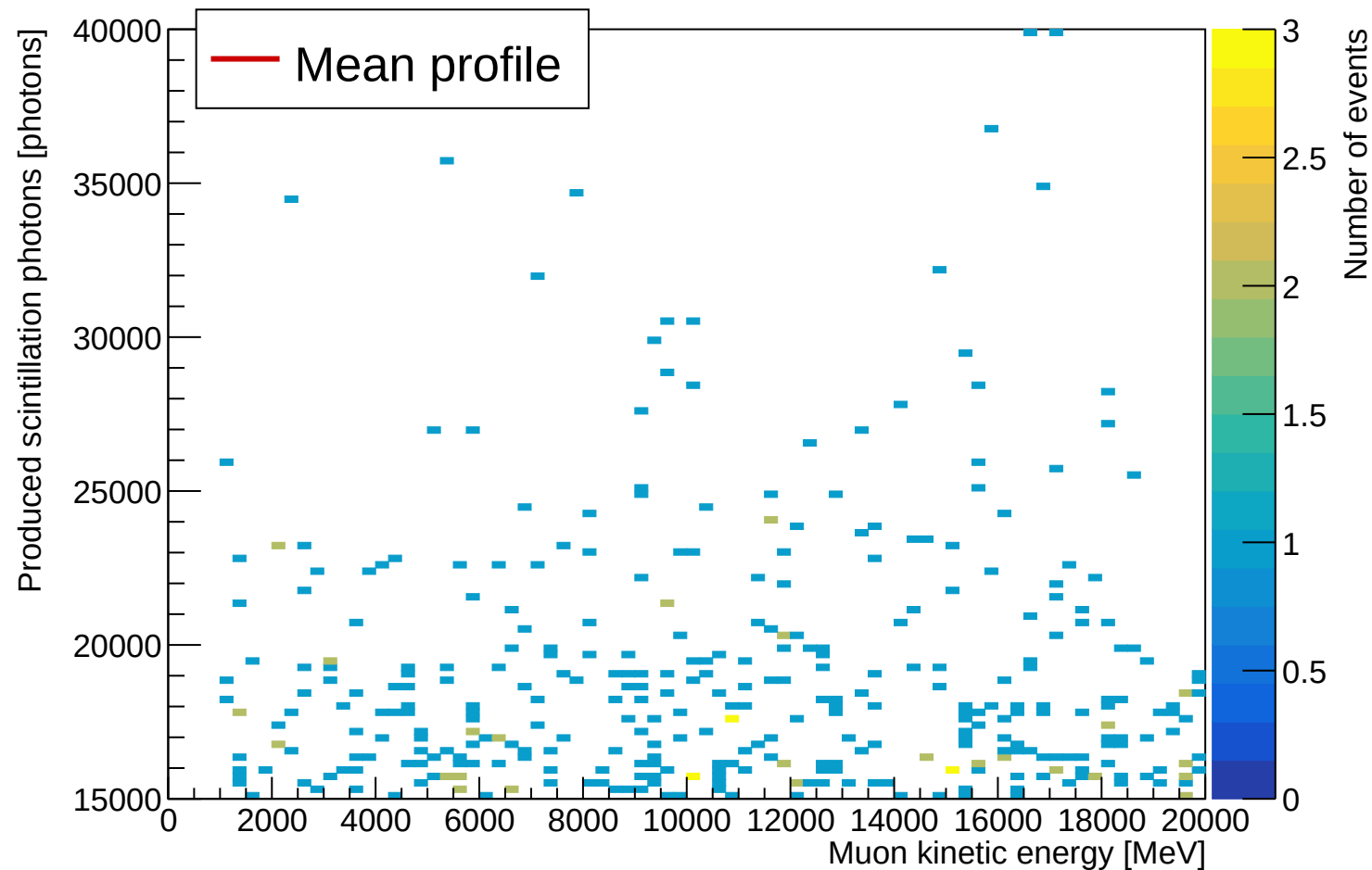
Scintillation-light production versus muon energy ( 20 \times 20 mm tile)
