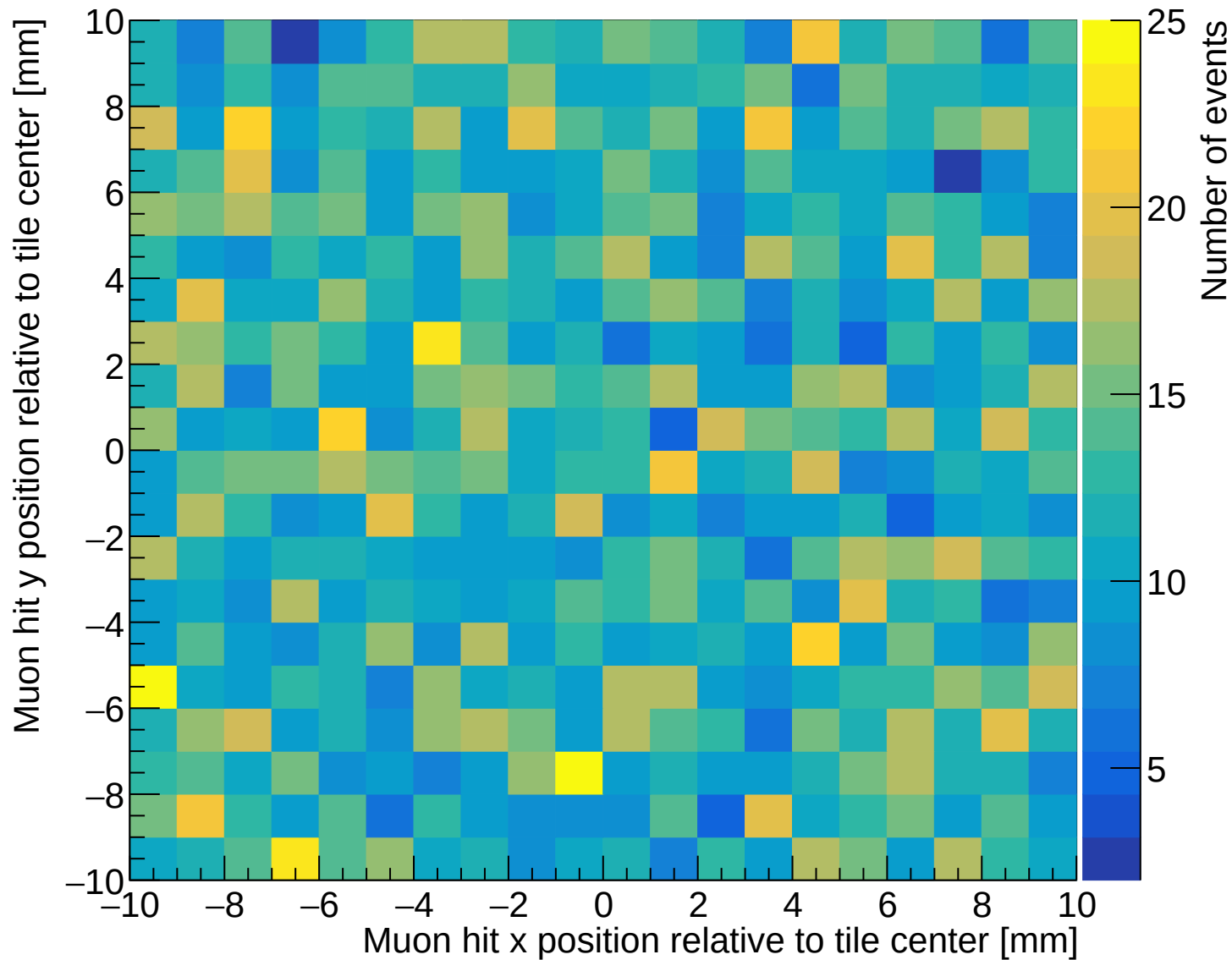
Simulated muon hit positions ( 20 \times 20 mm tile)
