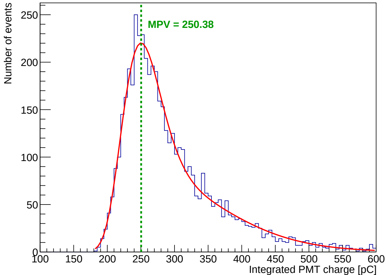
PMT charge distribution ( 20 \times 20 mm tile)
