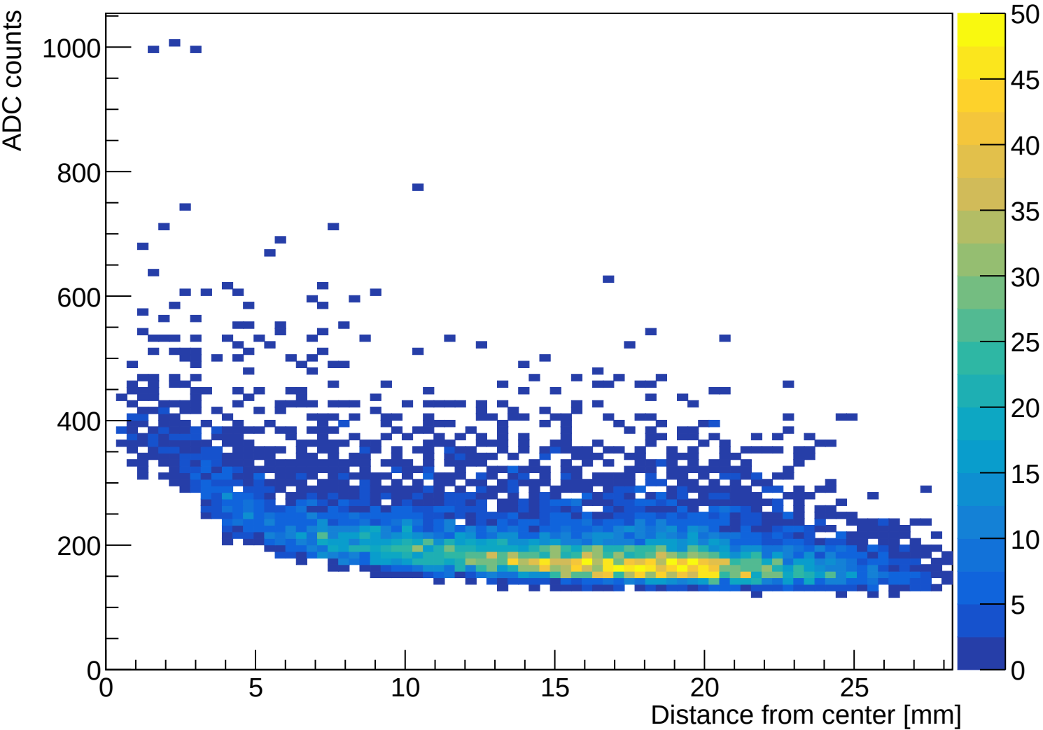
ADC response versus distance from tile center
