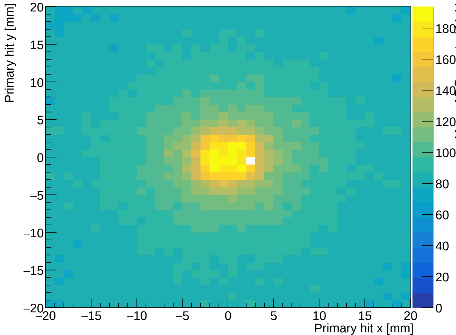
Energy-normalized ADC response across the tile
