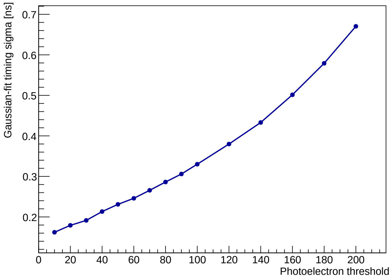
Timing Sigma vs Photoelectron Threshold
