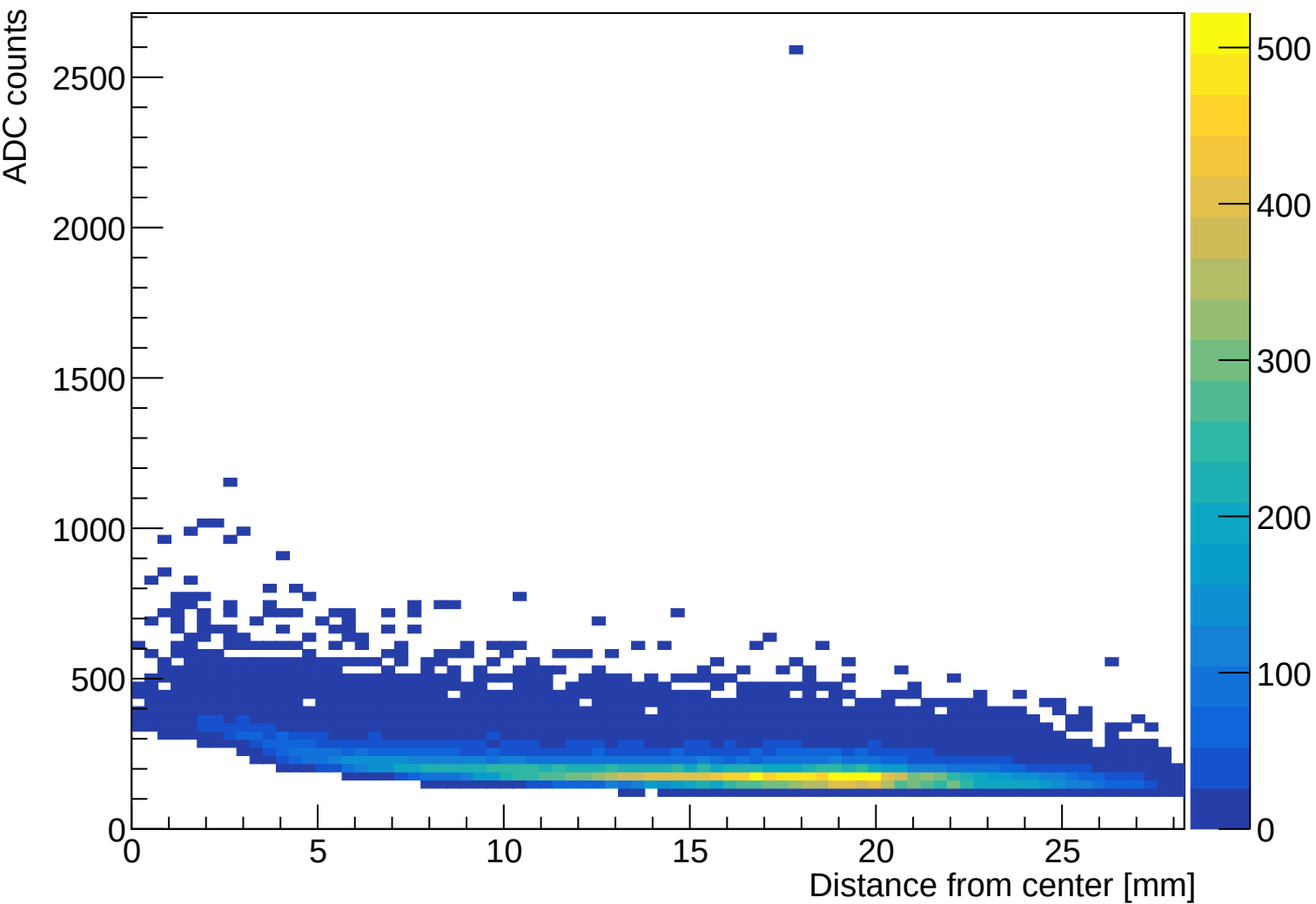
ADC response versus distance from tile center
