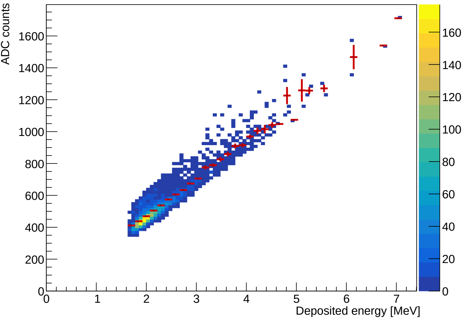
ADC response versus deposited energy
