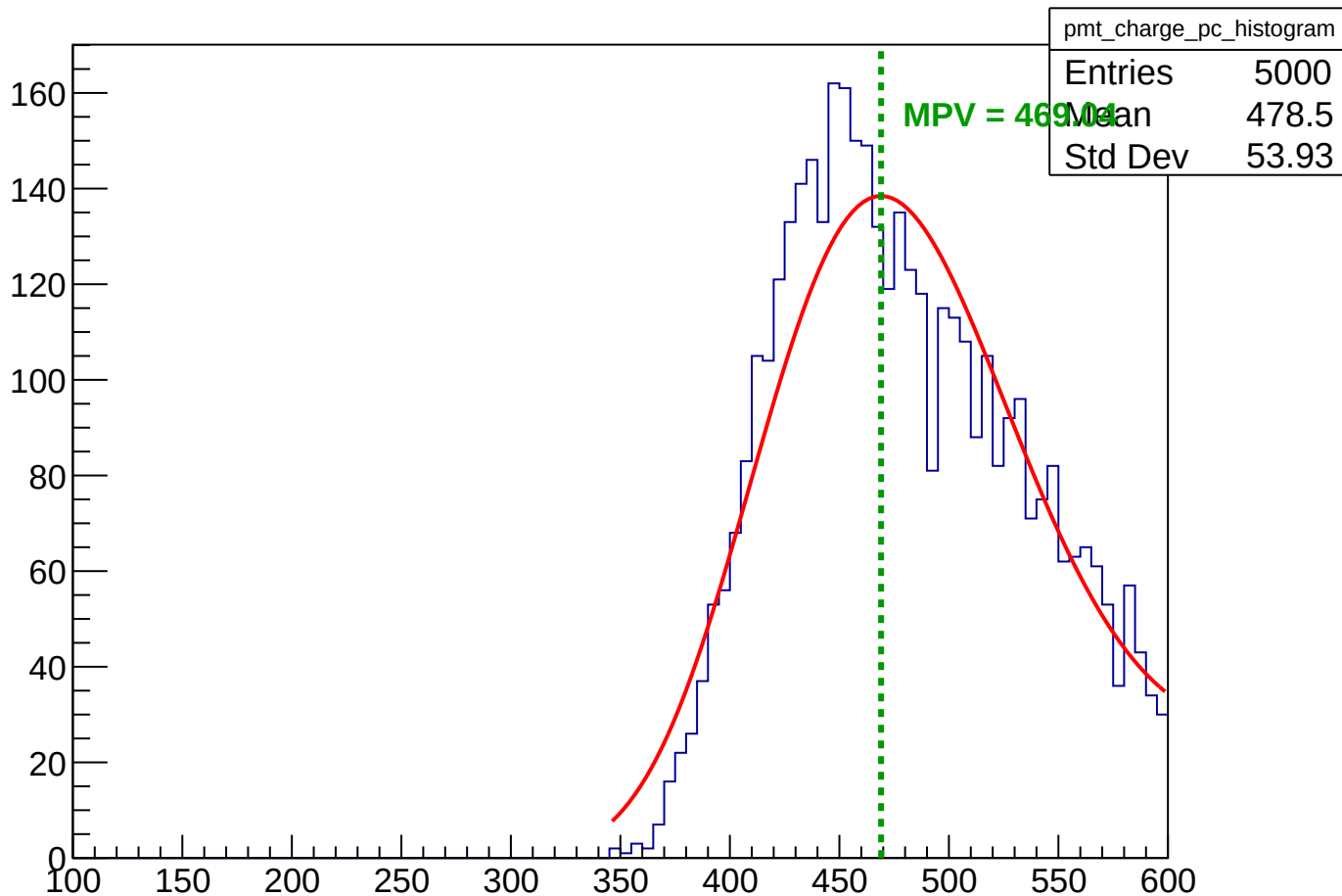
pmt_charge_pc_histogram
