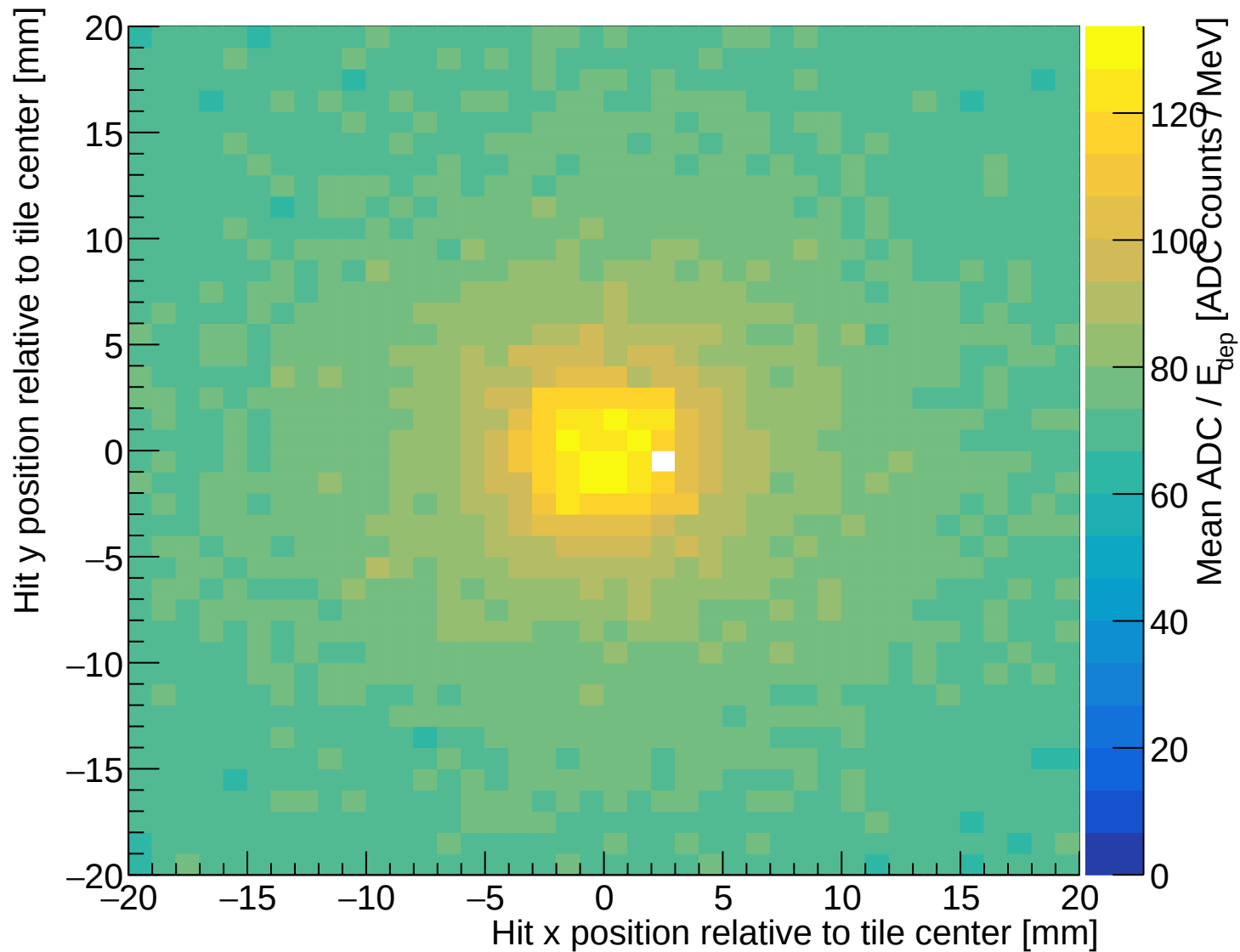
ADC response per deposited energy versus hit position (40 x 40 mm tile)
