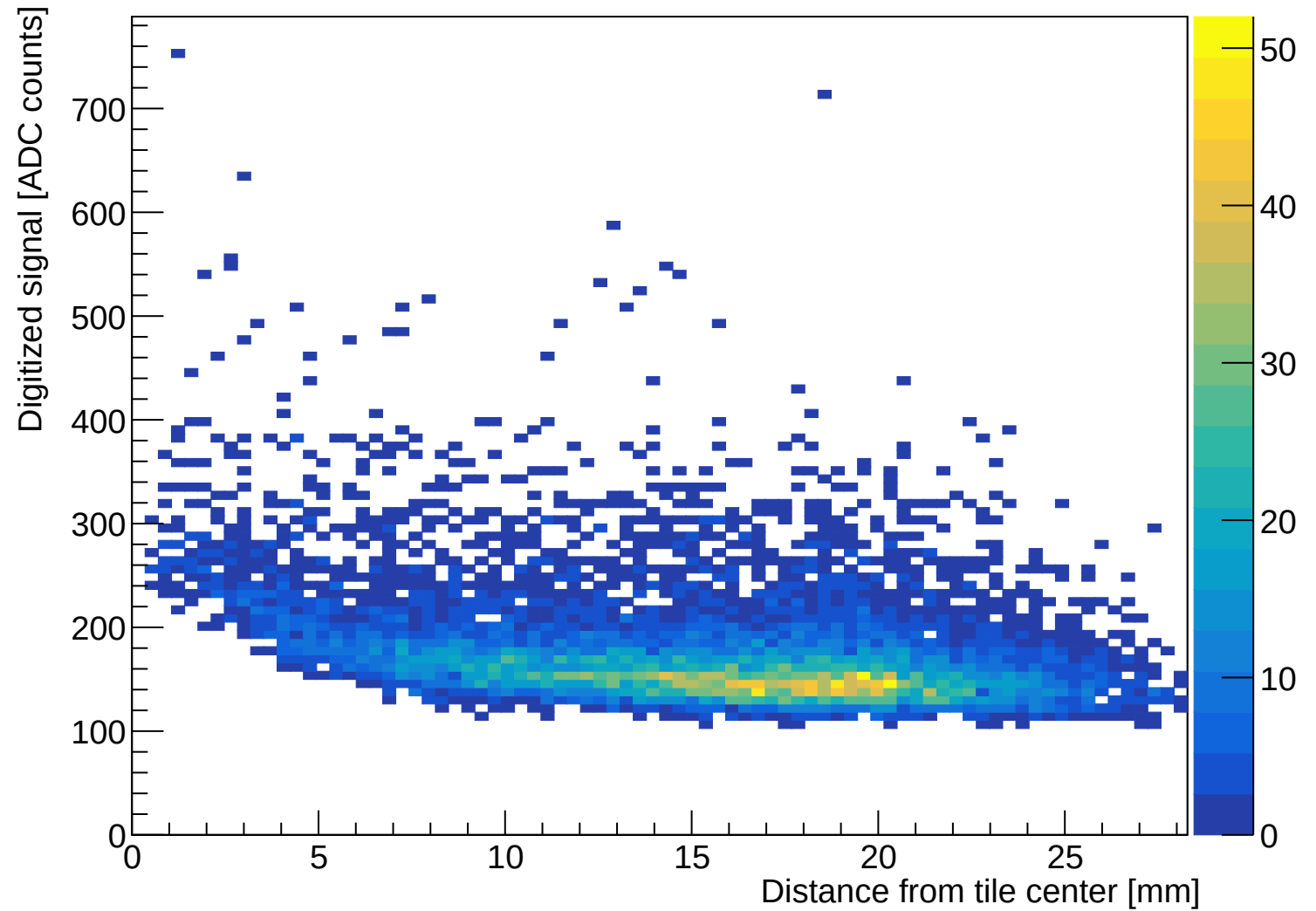
ADC response versus radial hit position (40 x 40 mm tile)
