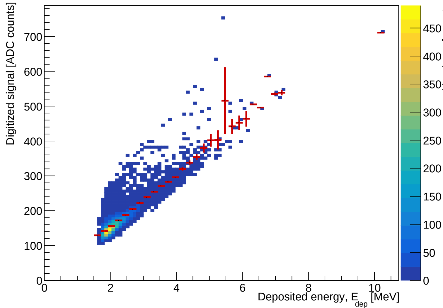
ADC response versus deposited energy (40 x 40 mm tile)
