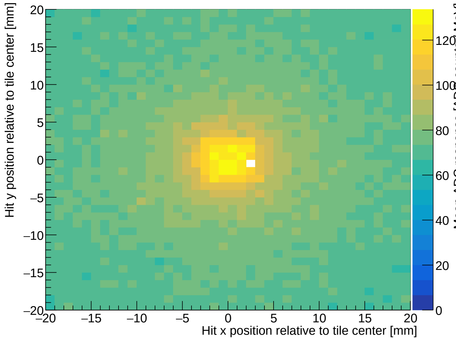
Mean energy-normalized ADC response versus hit position (40 x 40 mm tile)
