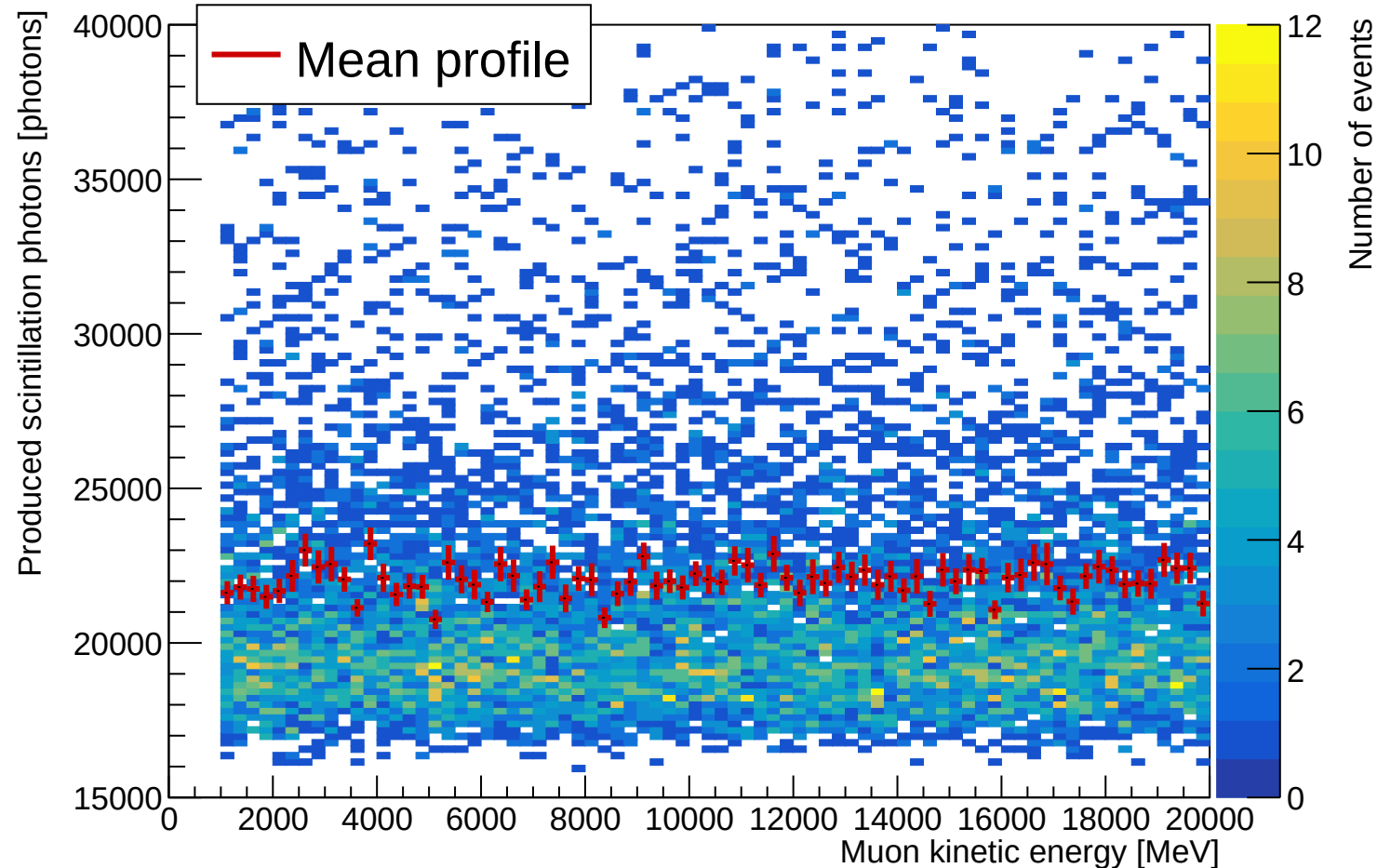
Scintillation-light production versus muon energy (40x40 mm tile)
