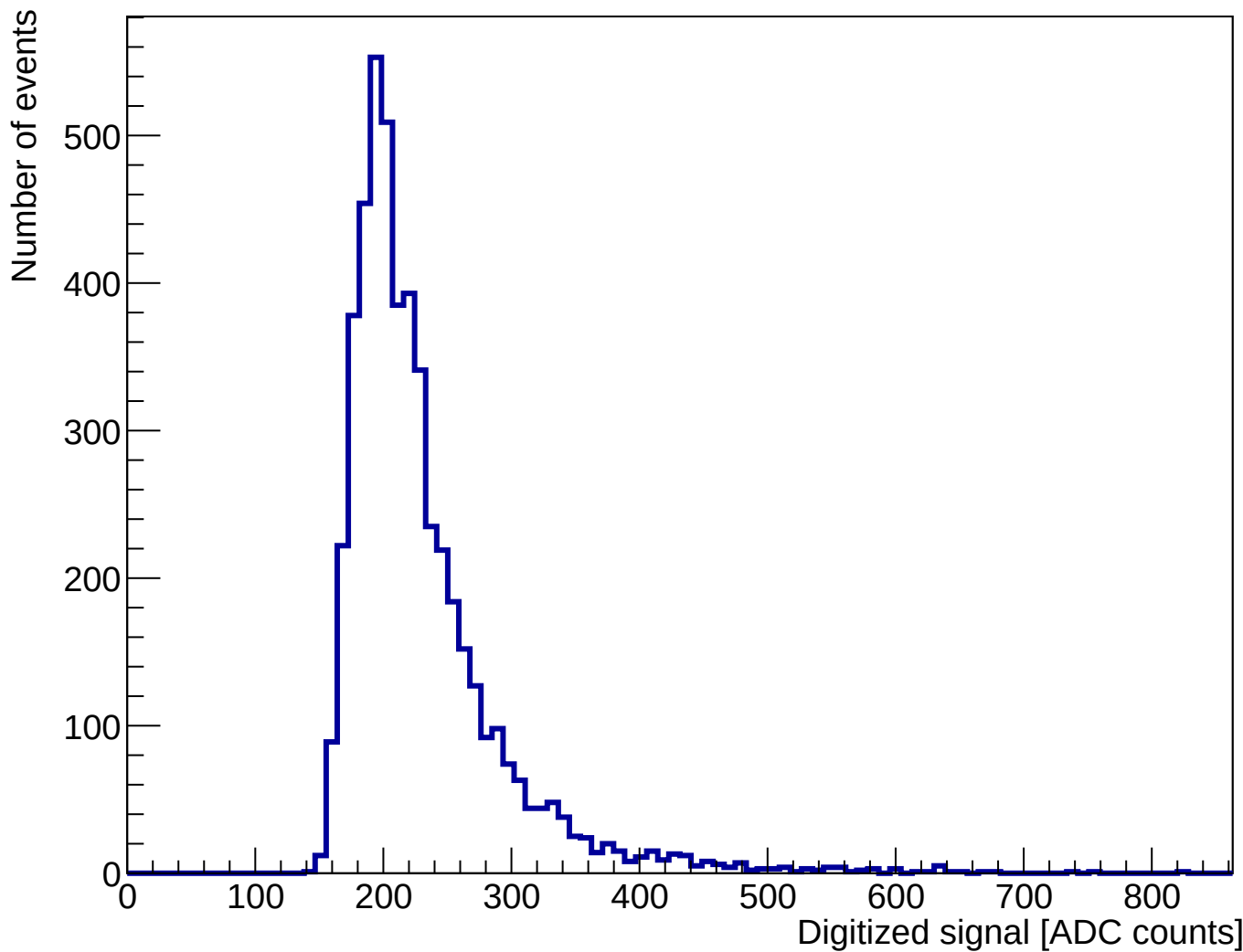
Digitized-signal distribution (20 x 20 mm tile)
