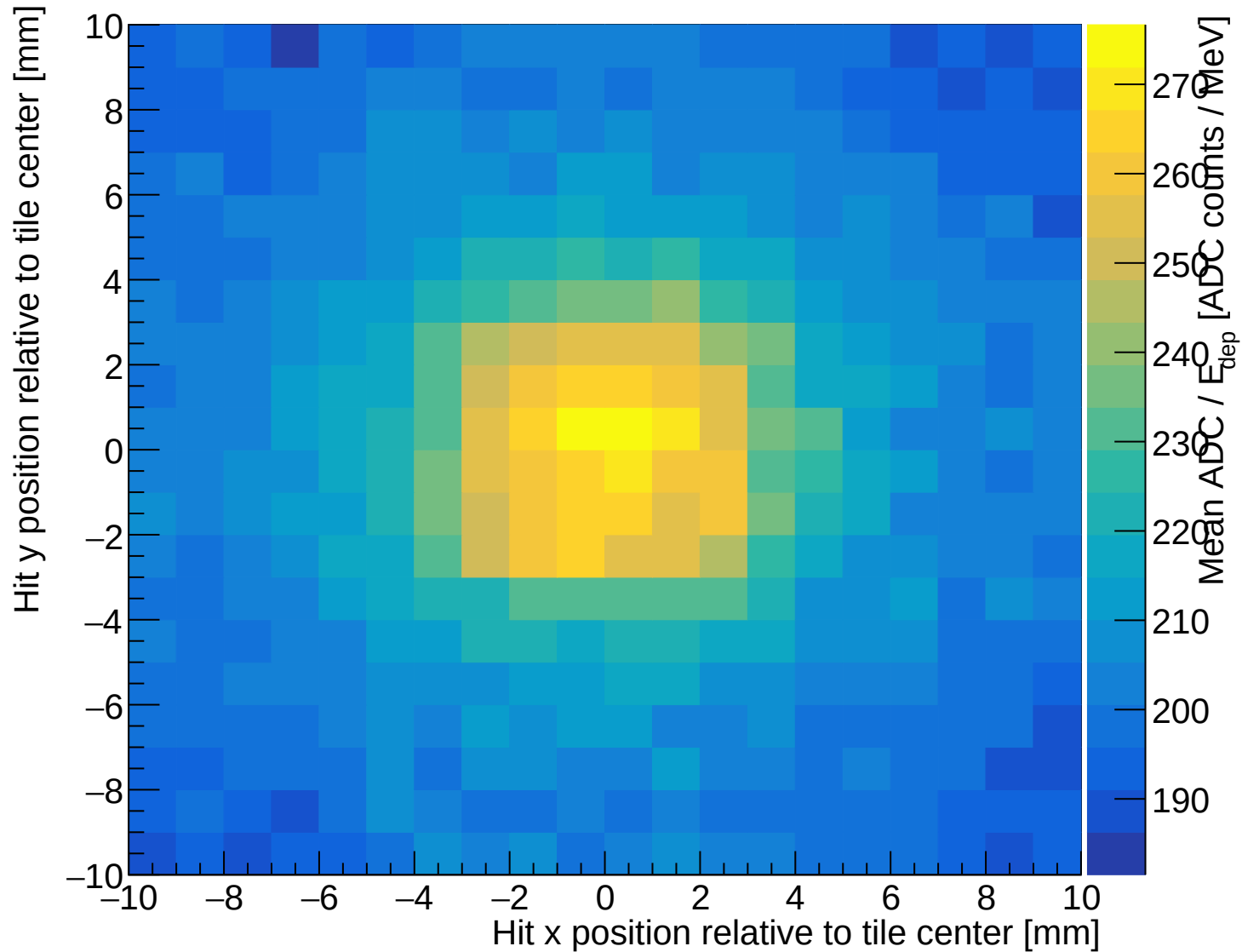
ADC response per deposited energy versus hit position (20 x 20 mm tile)
