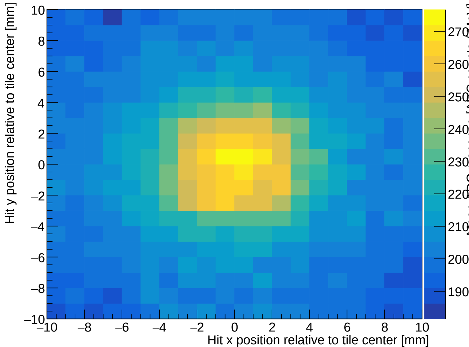
Mean energy-normalized ADC response versus hit position (20 x 20 mm tile)
