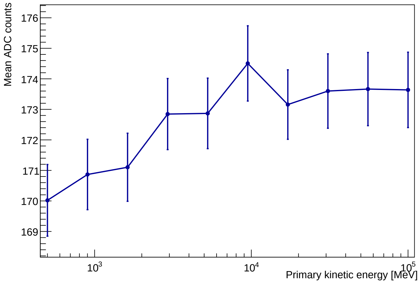
Mean ADC Counts vs Primary Energy: Muon
