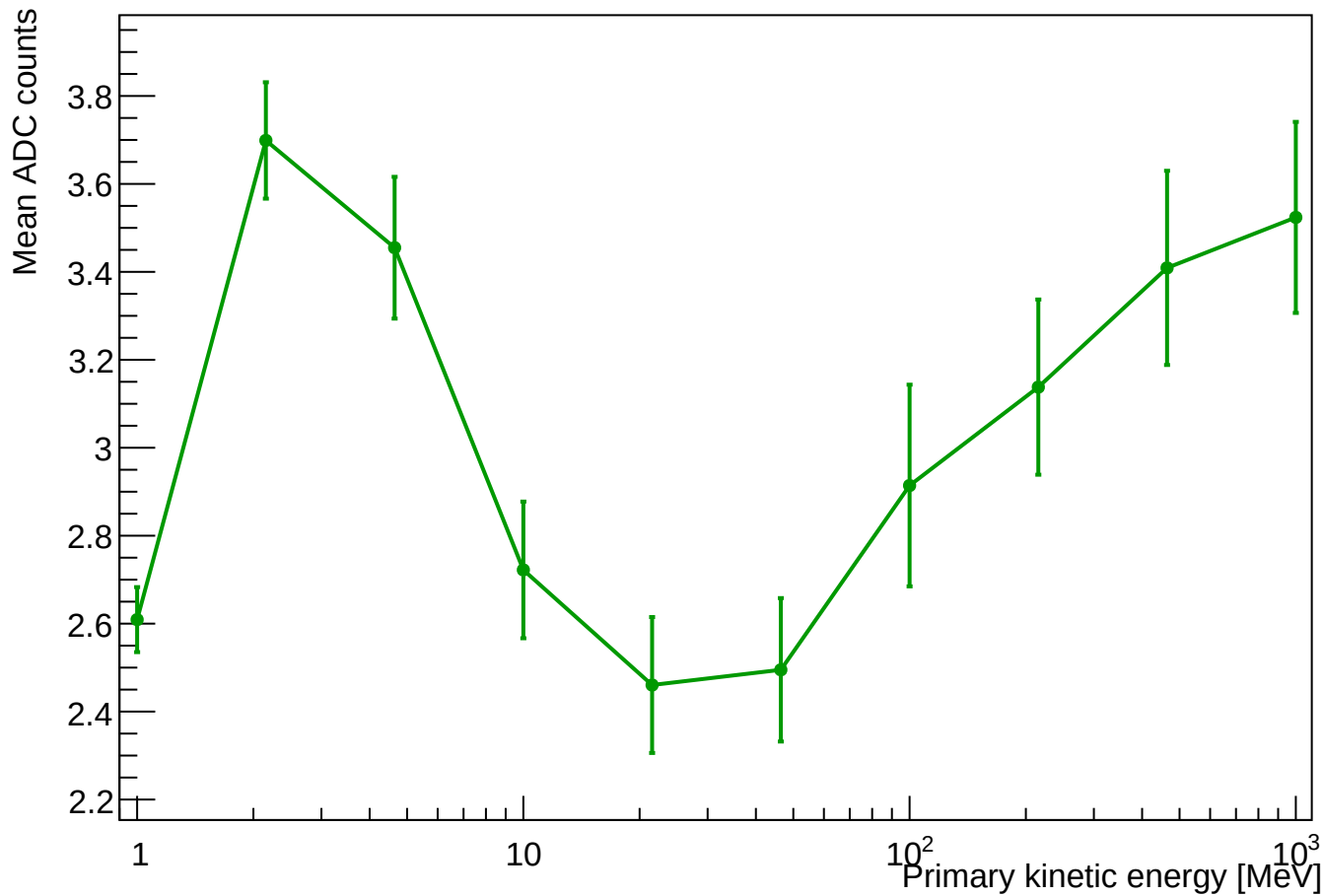
Mean ADC Counts vs Primary Energy: Photon
