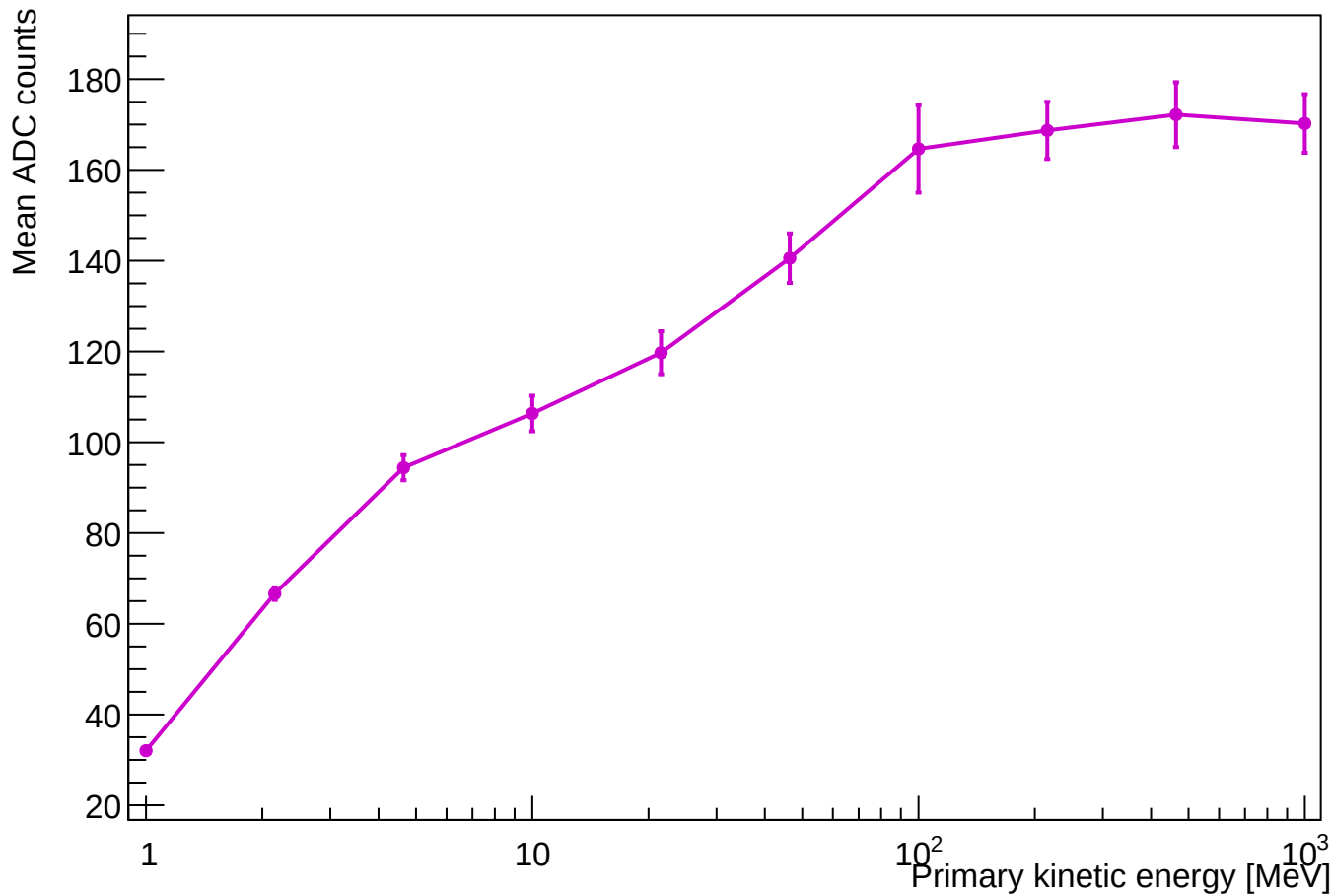
Mean ADC Counts vs Primary Energy: Photon (interacted)
