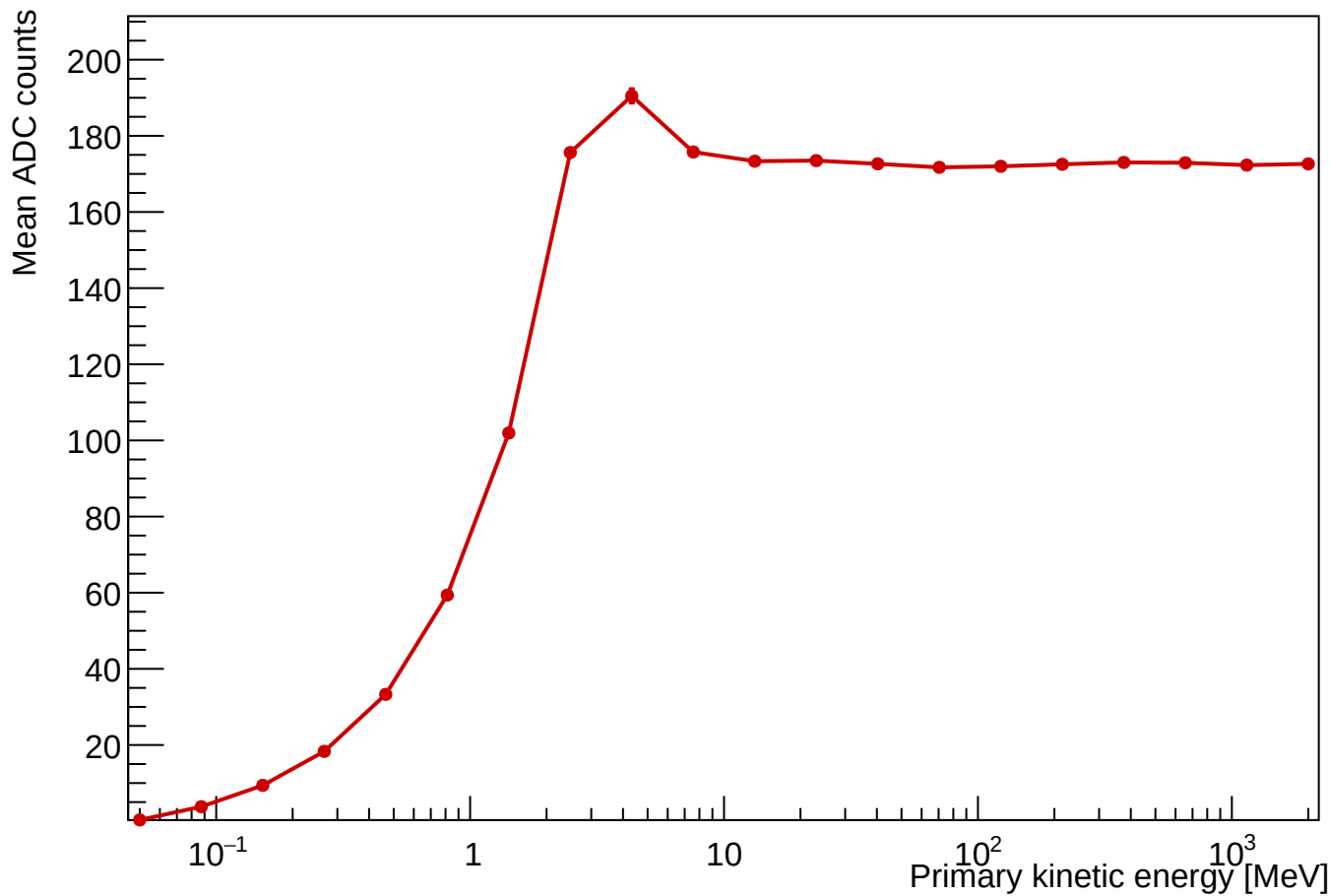
Mean ADC Counts vs Primary Energy: Electron
