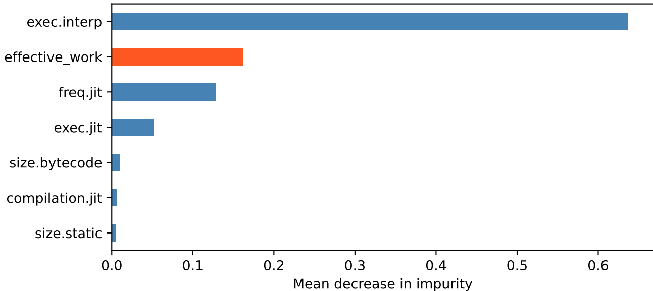
Feature importances for hot/cold classification (Random Forest)
