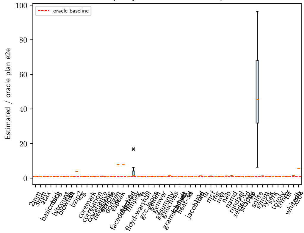
Plan quality: estimated vs oracle profile
