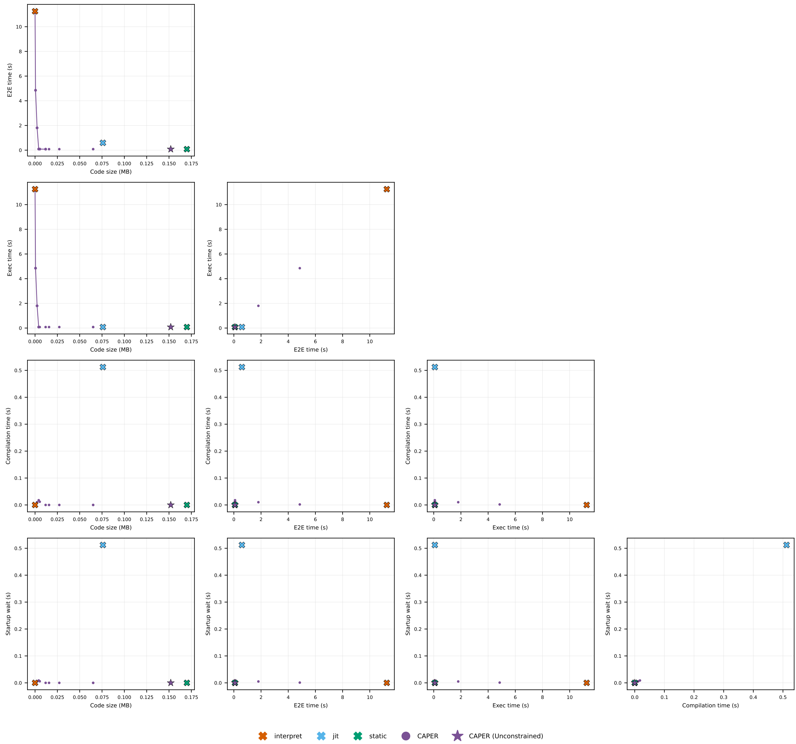
bitcount · bitcount: pairwise metric trade-offs
