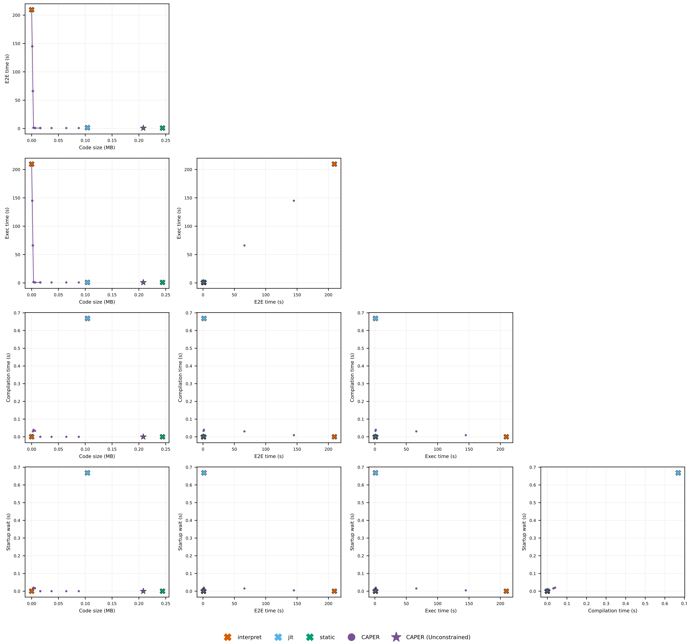
CG · CG: pairwise metric trade-offs
