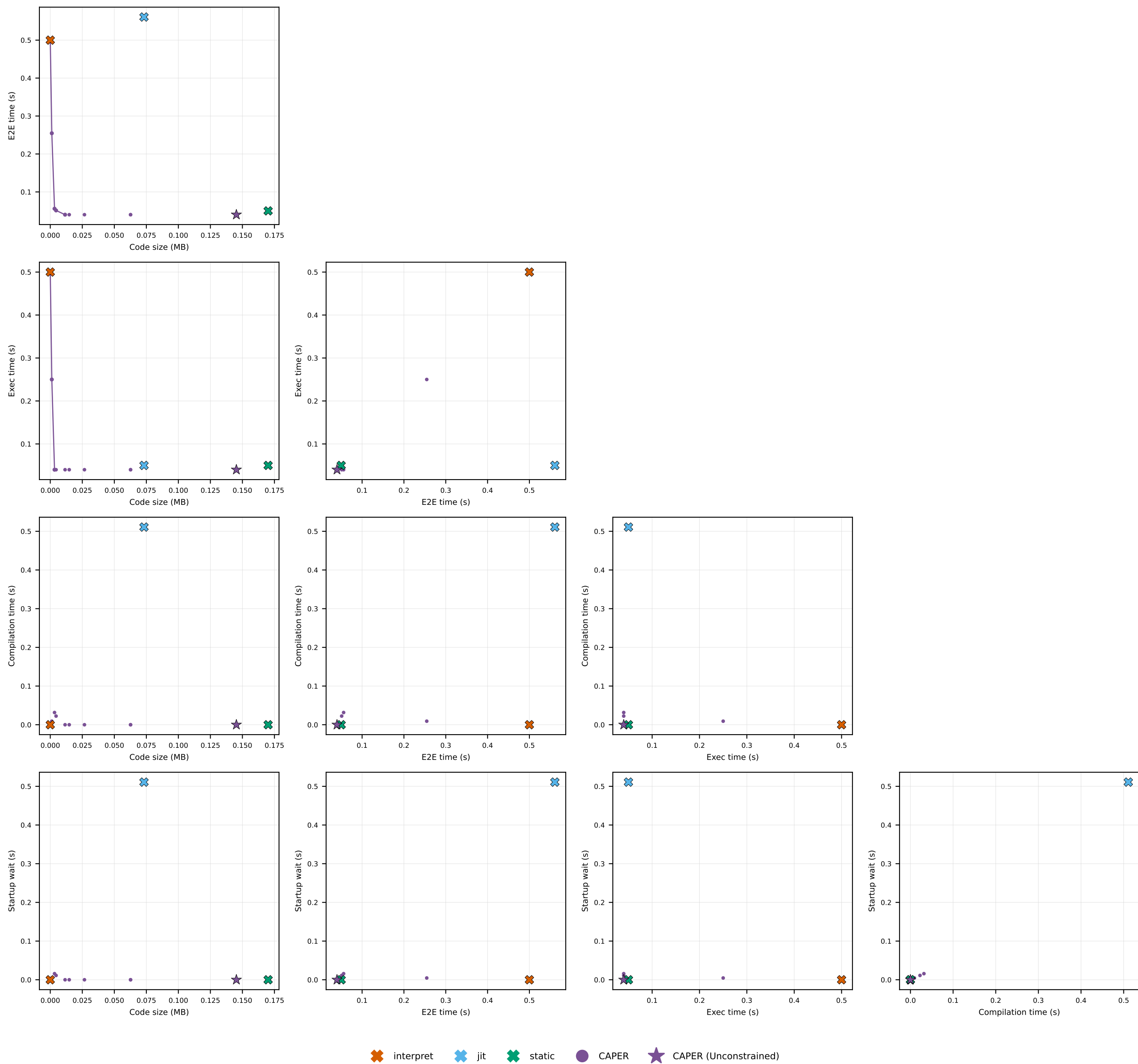
covariance · covariance: pairwise metric trade-offs
