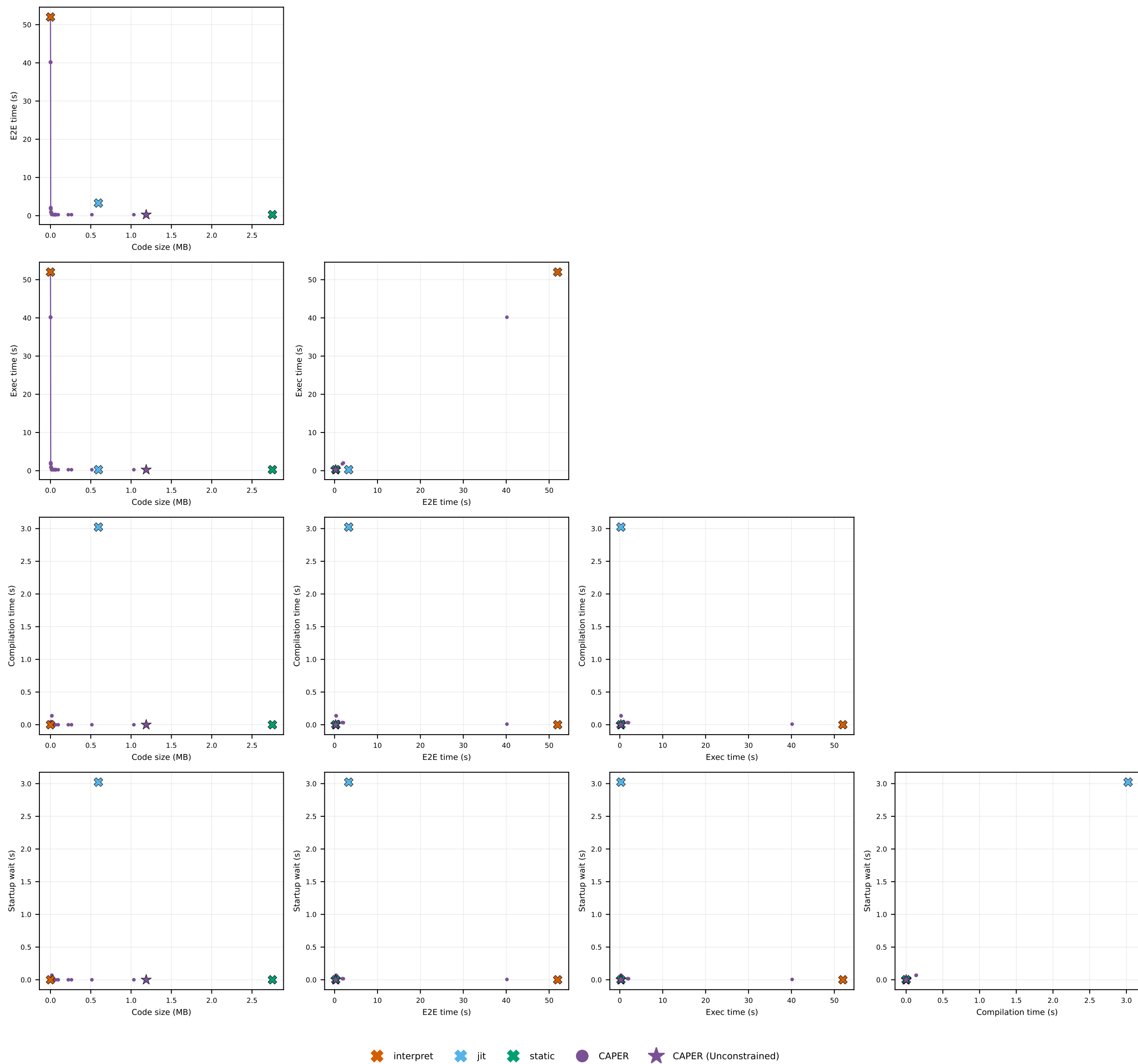
facetedetection · facedetection: pairwise metric trade-offs
