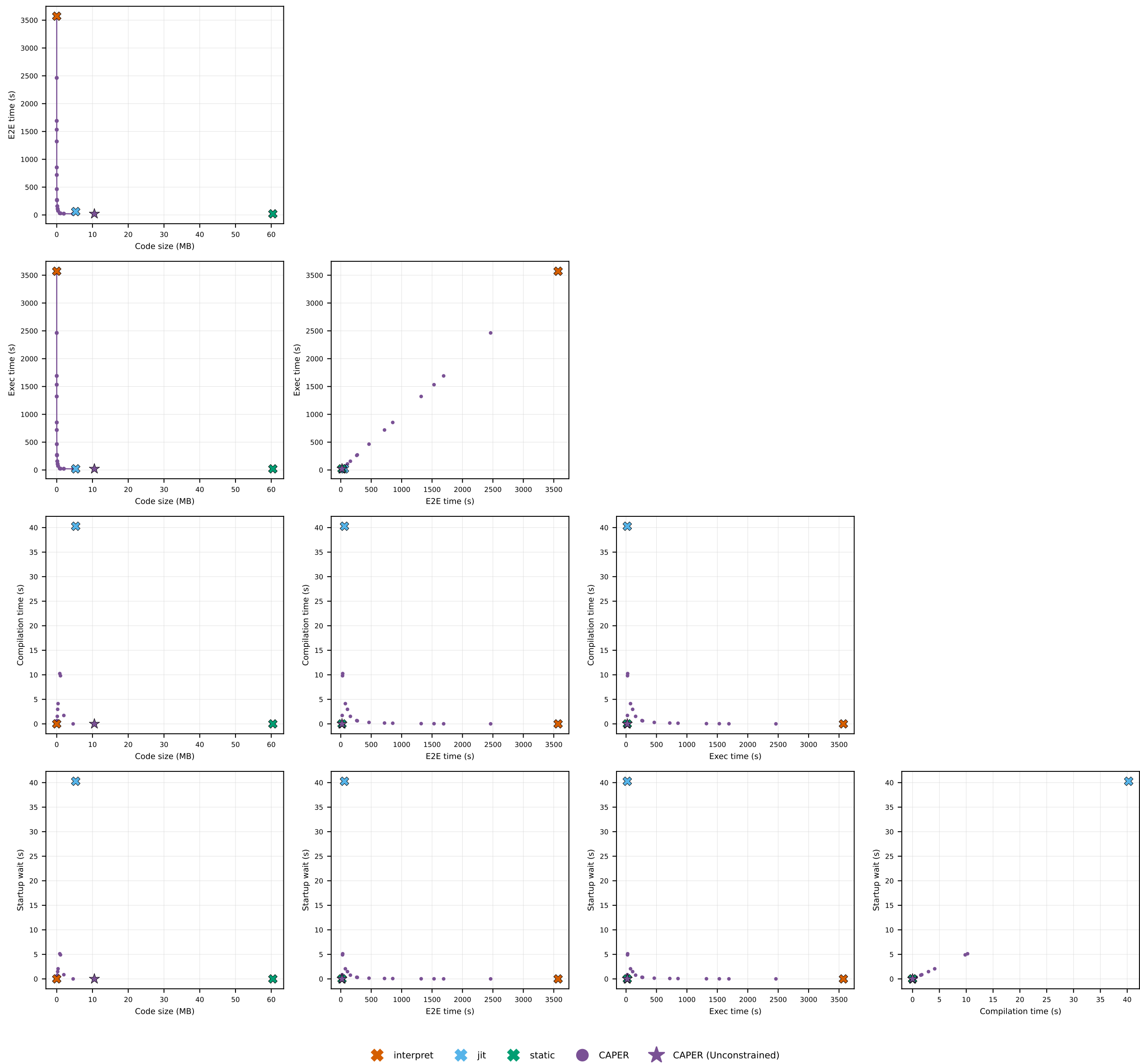
FFmpeg · mp4-resize-720p: pairwise metric trade-offs
