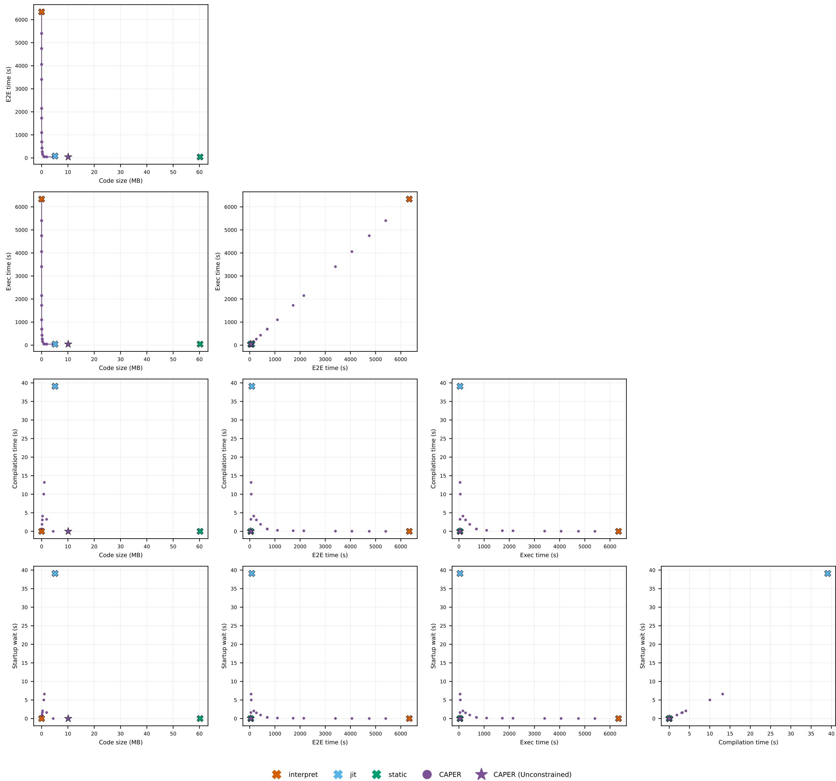
FFmpeg · mp4-speedup-2x: pairwise metric trade-offs
