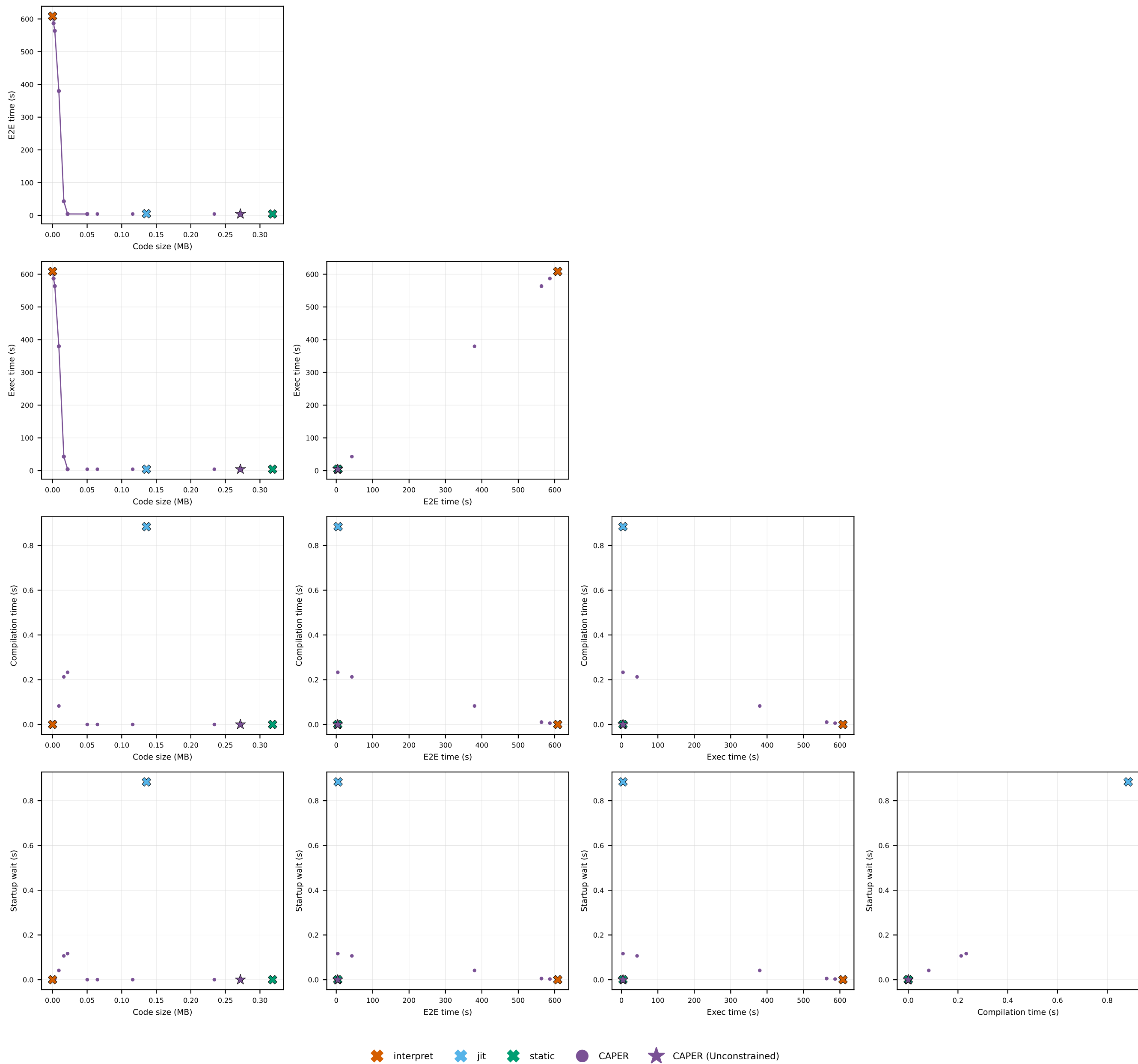
FT · FT: pairwise metric trade-offs
