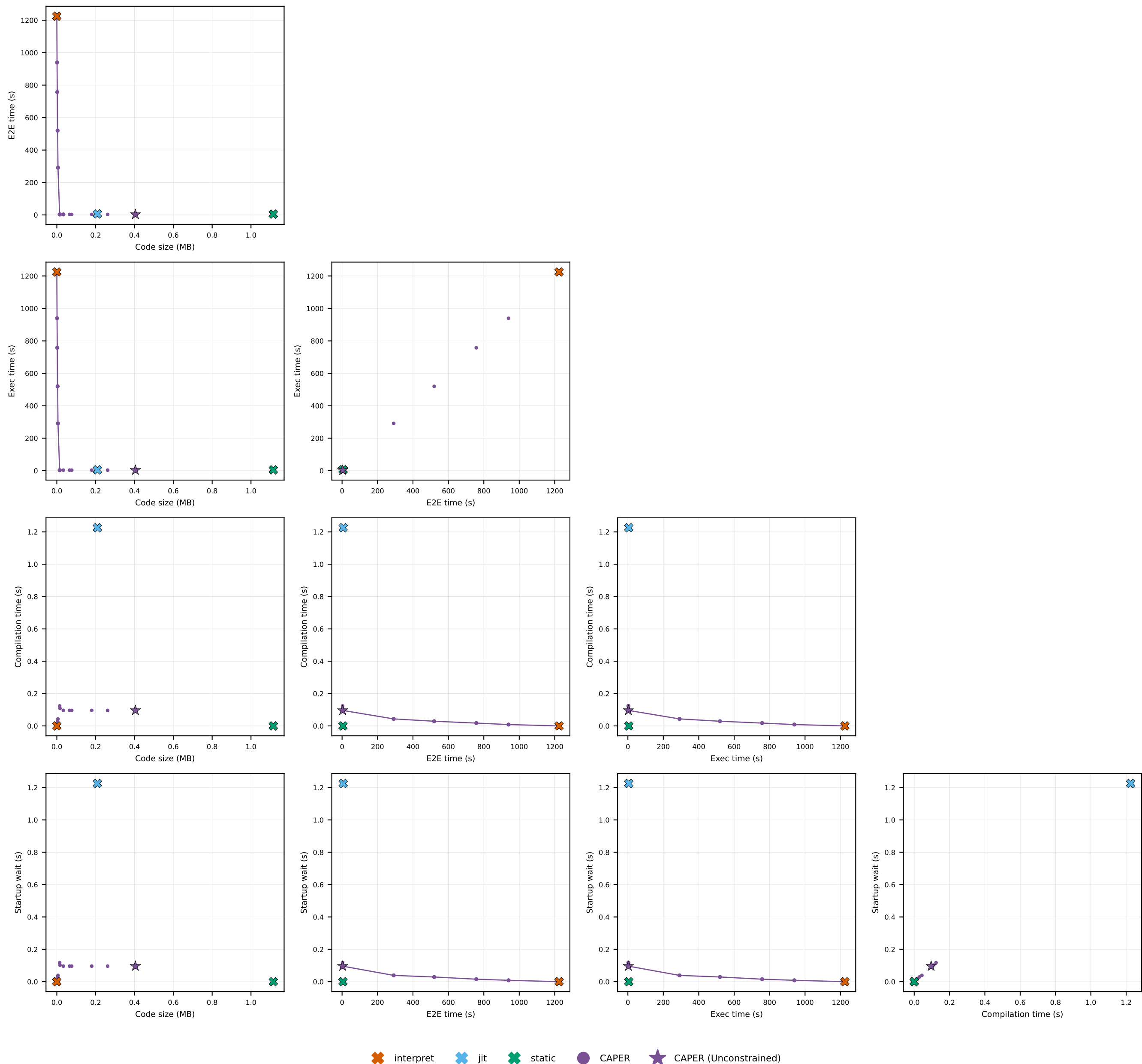
gcc-loops · gcc-loops: pairwise metric trade-offs
