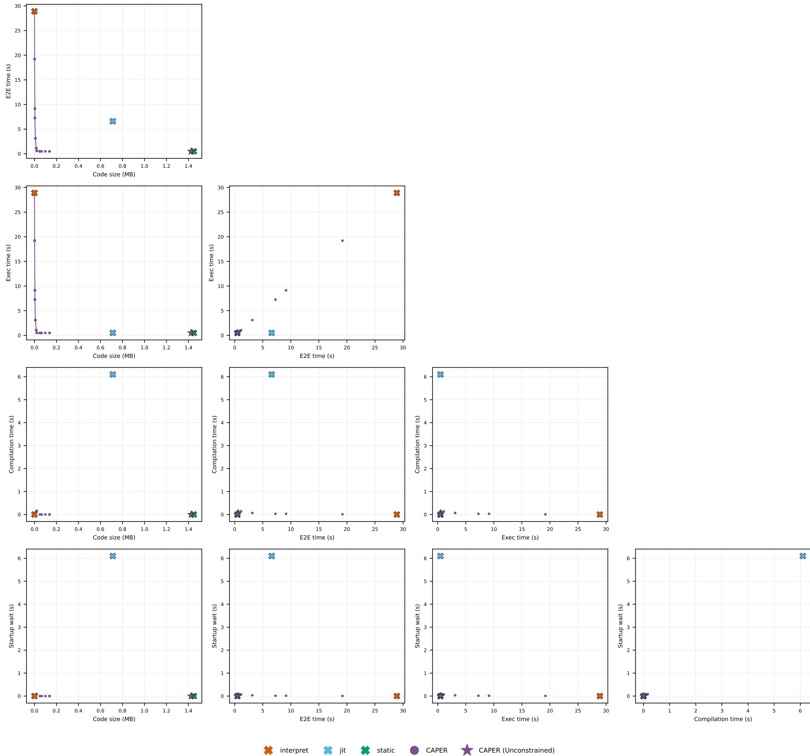
hashset · hashset: pairwise metric trade-offs
